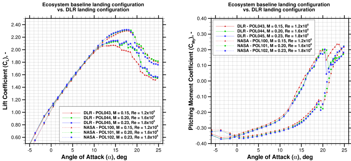
Figure 7 – Lift curve and pitching moment for NASA and DLR configuration and a Mach number variation.
