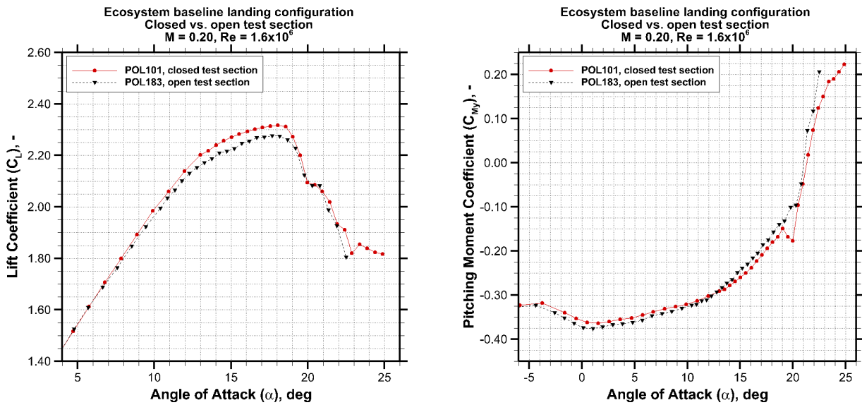
Figure 9 – Lift curve and pitching moment for the NASA configuration in the closed and \frac{3}{4} open test section
