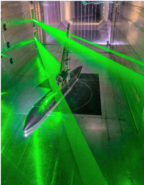
Figure 12 – Laser light sheets in the closed test section and their spanwise positions
