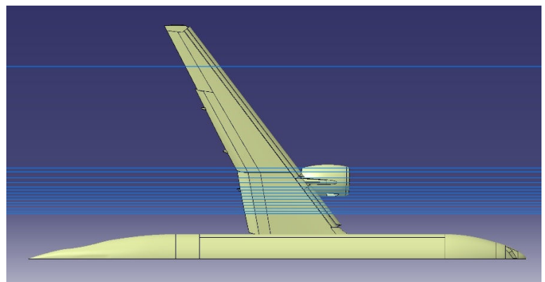
Figure 12 – Laser light sheets in the closed test section and their spanwise positions
