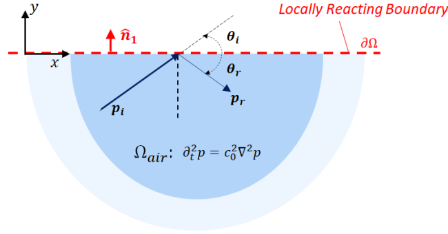
Figure 4 – Semi-infinite acoustic domain \Omega_{air} , expanding indefinitely along \pm x and \pm y , bounded on y = 0 by a locally-reacting boundary \partial\Omega , and definition of the incidence and reflection angles according to the convention adopted in this text.
