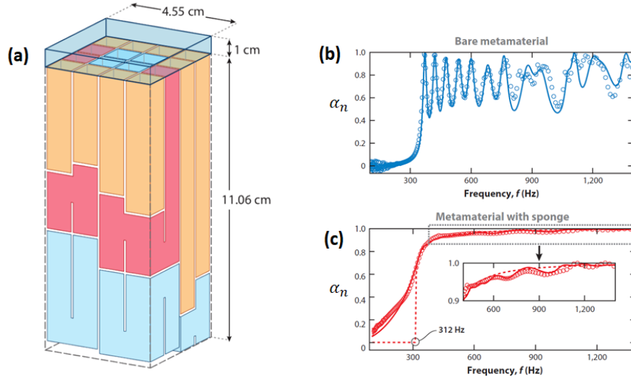
Figure 19 – Optimal absorber designed by [20], made of an array of channel-resonators (a), and its normal absorption \alpha_n performance without (b) and with (c) the addition of a sponge layer 1 cm thick.
