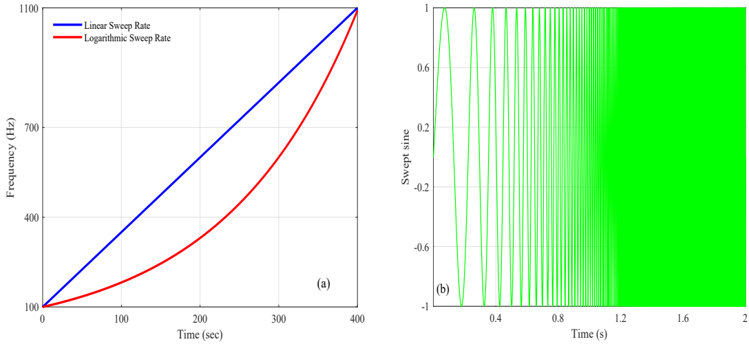
Figure 4 – (a) linear sweep rate vs. logarithmic sweep rate (b) time-sweep signal
