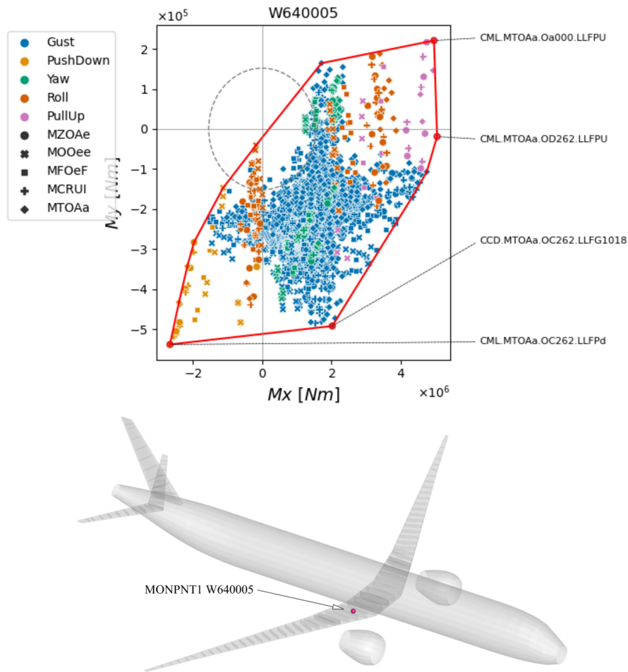
Figure 7 – Torsion ( M_y ) and bending moment ( M_x ) cut loads from steady and unsteady load cases (colors) and five different mass cases (symbols) resolved in a local coordinate system at inner monitoring station on the right wing.
