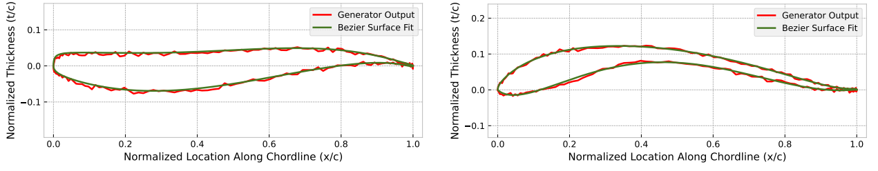
Figure 5 – Demonstration of the generator output smoothing with Bezier curve fitting for two airfoils generated from arbitrary latent vectors with values far from their respective means. Latent vectors are defined by \bar{z} = \bar{\mu} + \bar{w} \odot \bar{\sigma} , and the arbitrary weight vector \bar{w} is provided in the respective captions.
