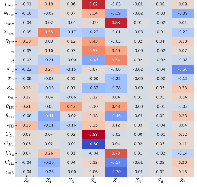
(b) 500 random samples \bar{z} \sim \mathcal{U}(\bar{\mu} - 2\bar{\sigma}, \bar{\mu} + 2\bar{\sigma})
