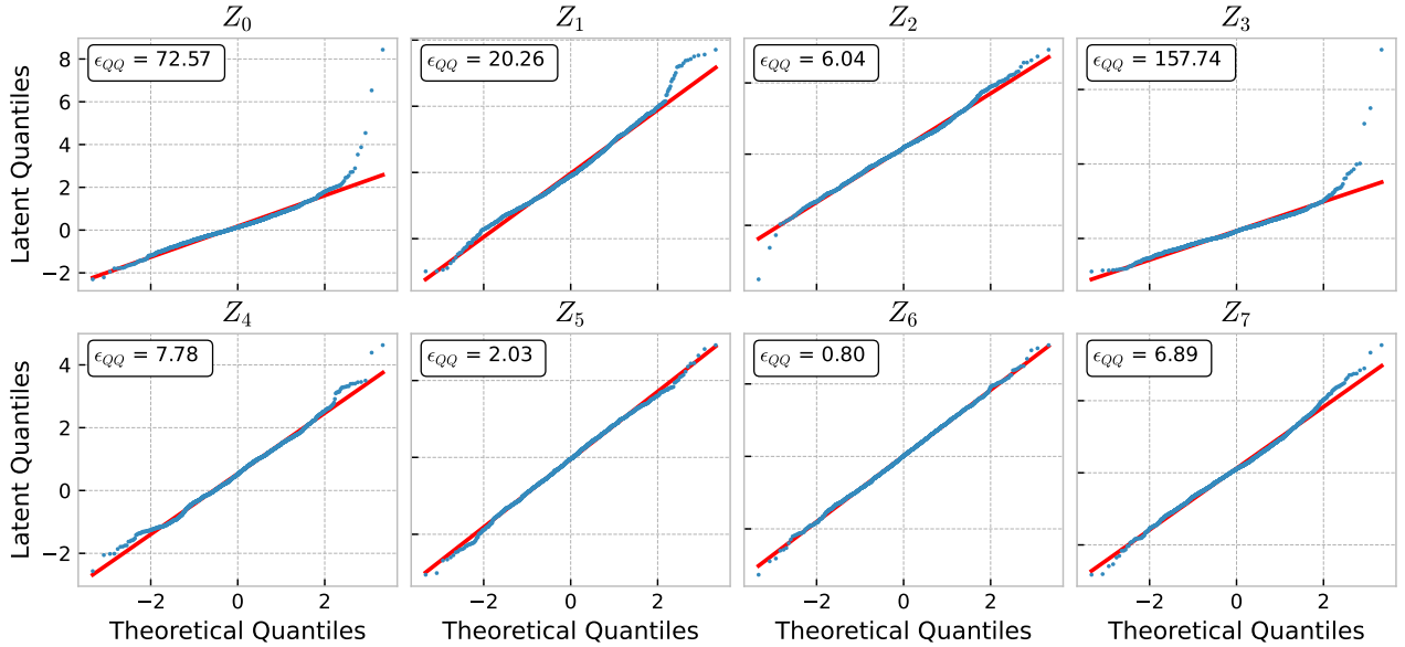
Figure 8 – Q-Q plot of the latent distributions compared to the Gaussian distribution pushed by the KL-divergence loss term during training.
