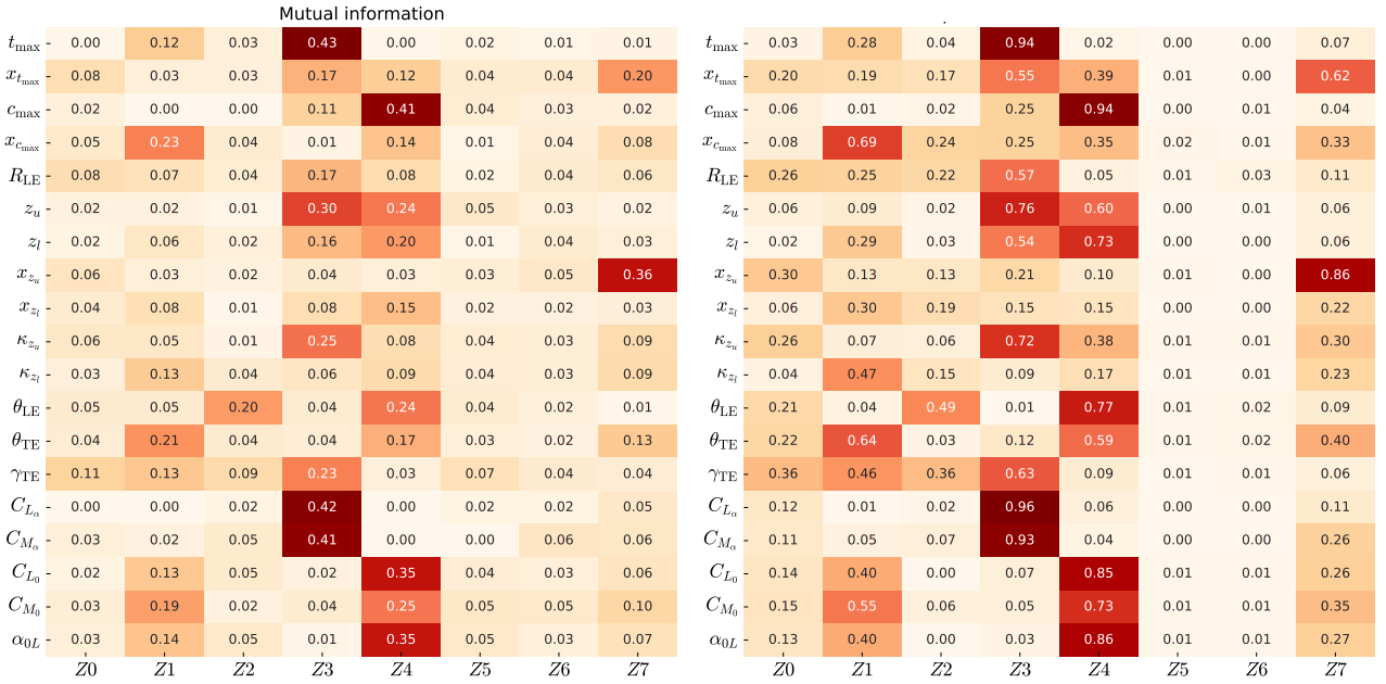
(a) Mutual Information matrix
