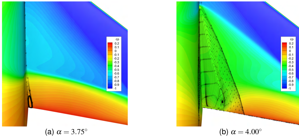
Figure 12 – Development of SoB separation for SA-neg at high angles-of-attack.
