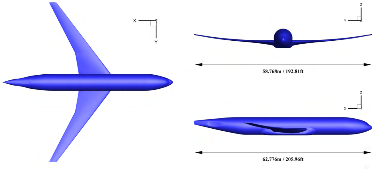
Figure 1 – NASA Common Research Model in Wing-Body configuration.
