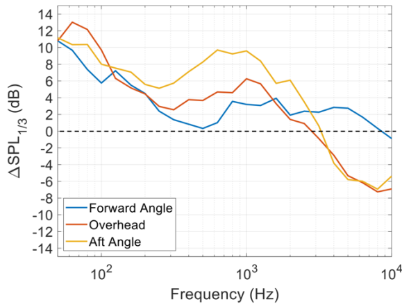
Figure 8 – 2022 reported results [14] difference of ANOPP-Research prediction minus flight data. High power condition.
