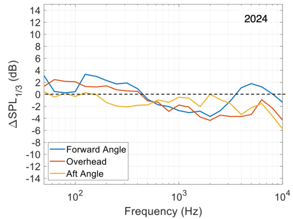
Figure 13 – Refined ANOPP-Research prediction minus flight data. All improvements (sections 4.1-4) including the PAASc fan broadband scattering prediction replacing previous LSAF-PAA-data-based method. High power condition.
