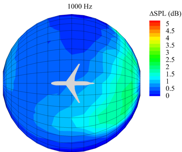
Figure 3 – PAASc-predicted scattered field of inlet-radiated fan broadband noise from the location of the inlet plane on the left (lower) wing.
