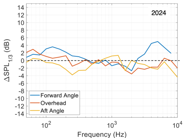
Figure 15 – Refined ANOPP-Research prediction minus flight data. All improvements (sections 4.1-4) included. Mid power condition.
