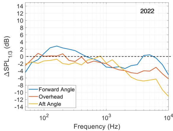
Figure 16 – Comparison of the best 2022 ANOPP-Research prediction with flight data and only adding the more accurate liner areas (section 4.1). Low power condition.
