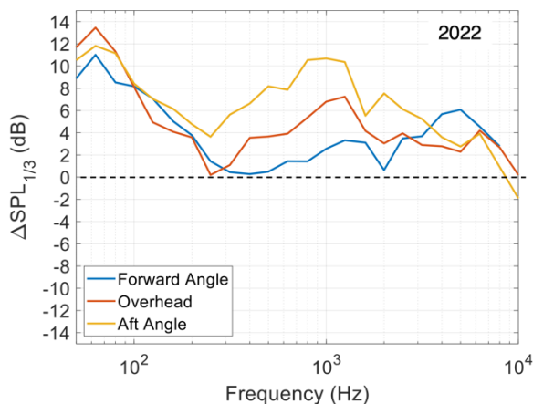
Figure 14 – Comparison of the best 2022 ANOPP-Research prediction with flight data and only adding the more accurate liner areas (section 4.1). Mid power condition.
