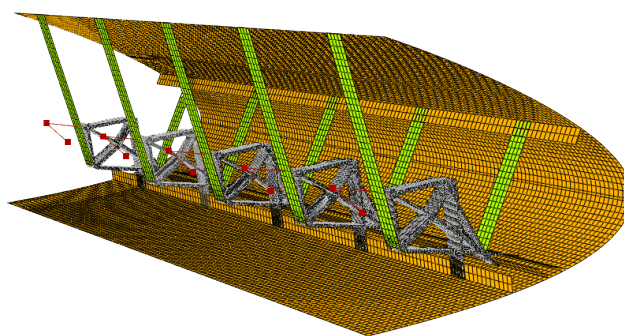
Figure 11 – 3D FEM model of the full-scale prototype.
