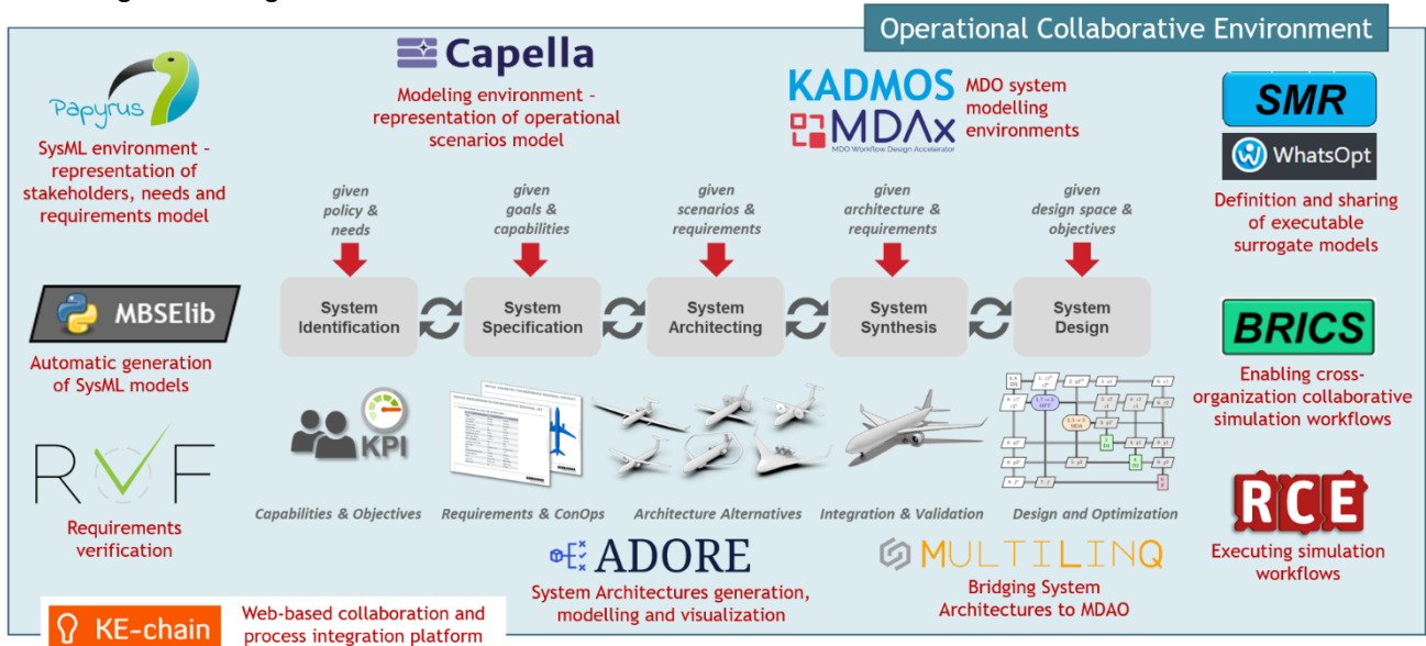
Figure 5 – Schema with the overview of the technologies of the AGILE 4.0 MBSE-MDO Development Framework. The implementation of the framework is named Operational Collaborative Environment (OCE).
