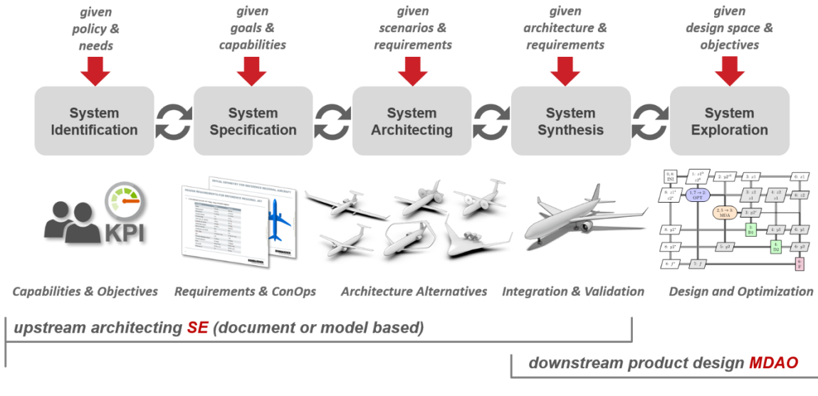
Figure 2 – The AGILE 4.0 MBSE-MDAO Development Framework: “upstream architecting SE” and “downstream product design MDAO” phases (adapted from [3]).
