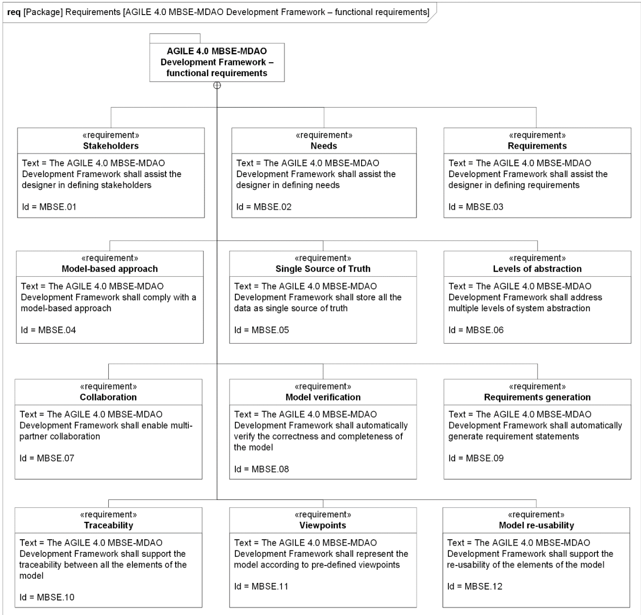
Figure 4 – SysML Requirements Diagram representing part of the requirements of the AGILE 4.0 MBSE-MDAO Development Framework (adapted from [9]).
