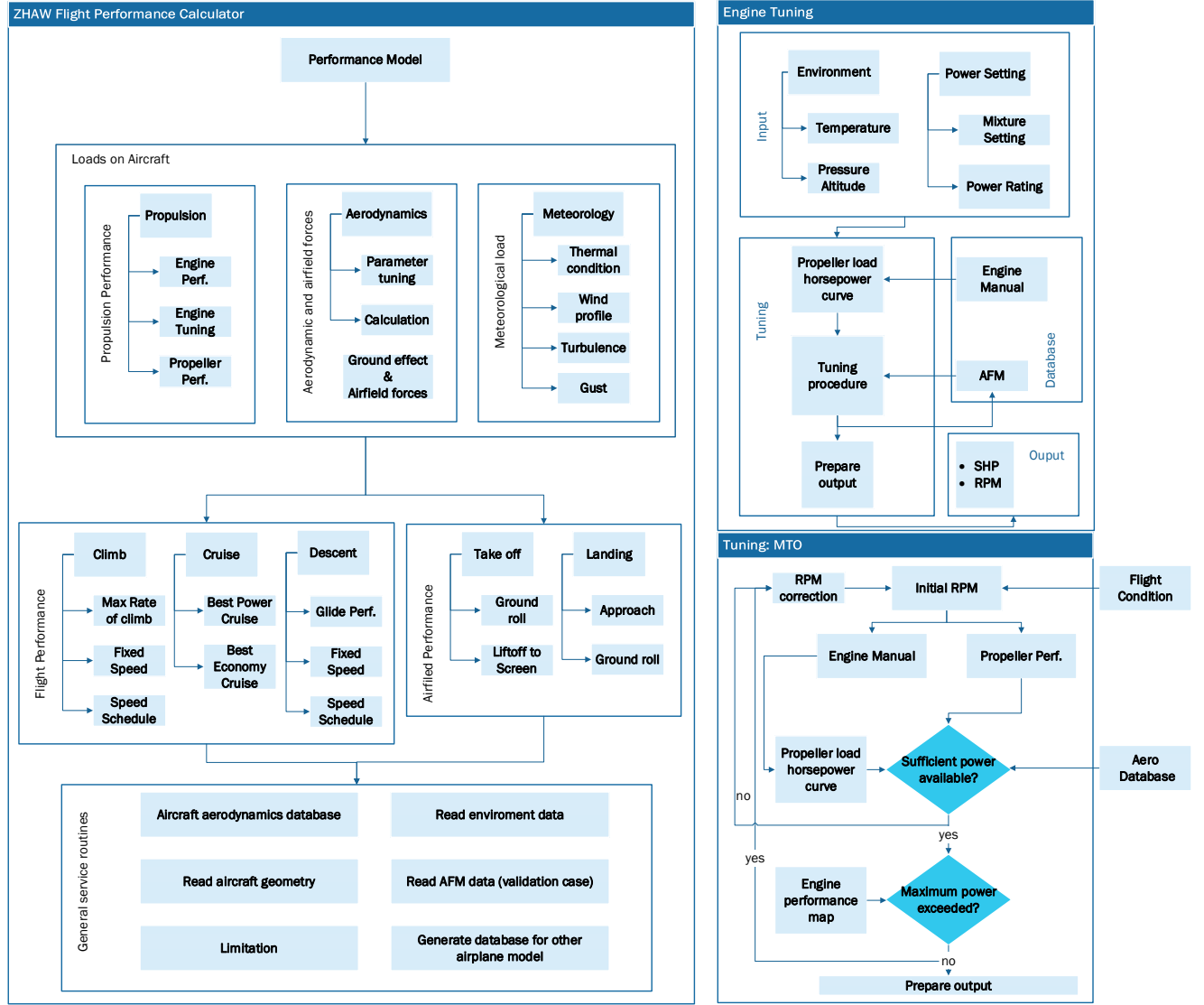
Figure 2 – Overview of flight performance calculator
