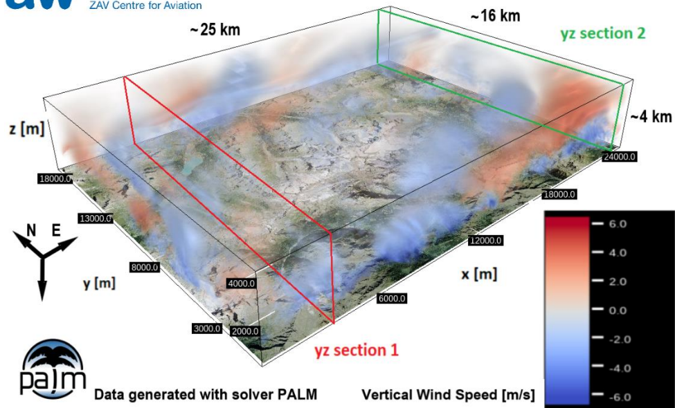
Figure 10 – 3D vertical wind field generated with PALM
