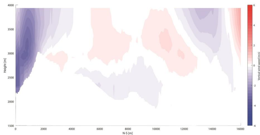
Figure 11 – Y-Z cross section 1 at 777799 E [CH 1903+] of the vertical wind field from PALM (upper) and kriged COSMO data (low)
