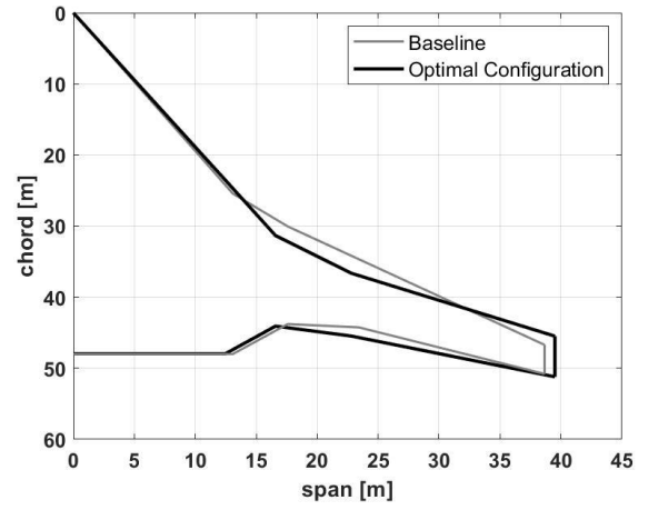
Figure 10 – Planform comparison for minimizing C_D .
