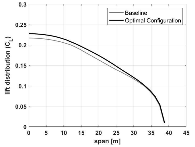
Figure 18 – Lift-distribution comparison E_{ff} and OEW optimisation – Configuration B.
