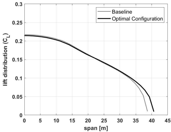
Figure 7 – Lift distribution comparison for maximizing E_{ff} .
