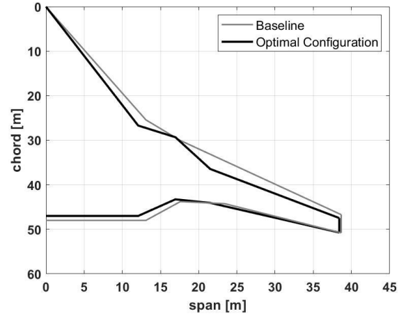
Figure 12 – Planform comparison for minimizing OEW.
