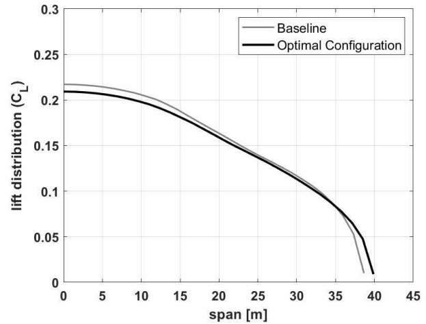
Figure 15 – Lift-distribution comparison E_{ff} and C_D optimisation – Configuration A.
