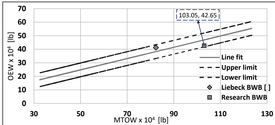
Figure 25 – Linear regression for OEW versus MTOW.
