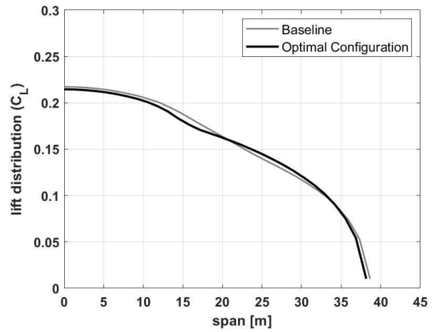
Figure 21 – Lift-distribution comparison C_D and OEW optimisation – Configuration C.
