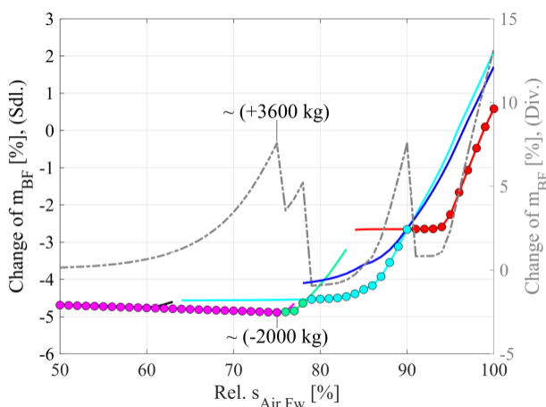
Figure 6: Reduction of burned fuel for DPP planning with formation benefits, 22.04.2012
