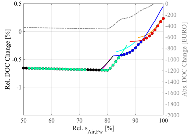
Figure 12: DOC reduction for max. benefit optimization, 04.08.2012
