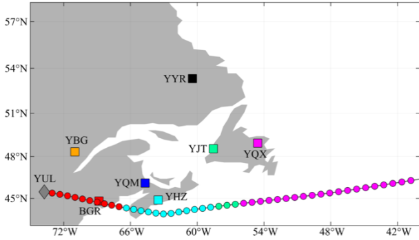
Figure 4: Follower track, potential DEC points assigned to ERA with minimum m_{TF} , 22.04.2012
