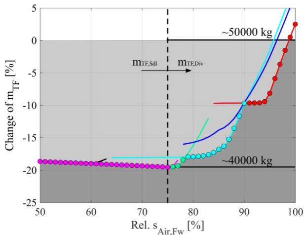
Figure 5: Required trip fuel according to DPP compared to a conventional fuel planning, 22.04.2012
