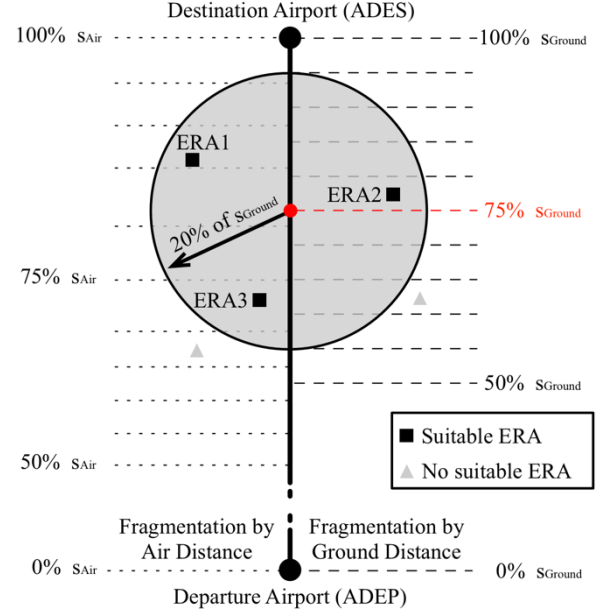
Figure 2: Area of suitable ERA airports and applied route fragmentation by air distance
