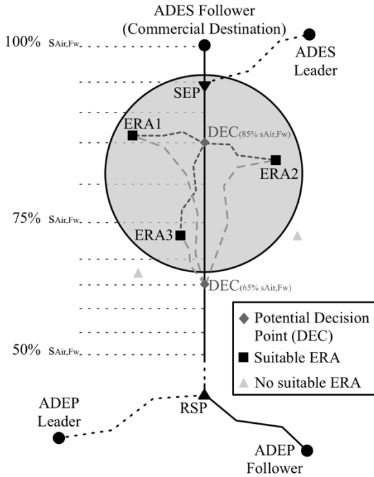
Figure 3: Formation route from the perspective of DPP flight planning
