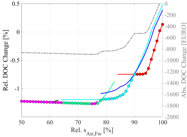
Figure 10: DOC reduction for max. benefit optimization, 22.04.2012
