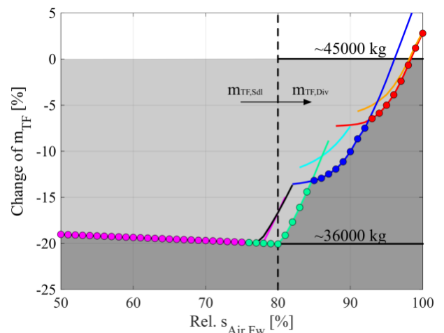
Figure 8: Required trip fuel according to DPP compared to a conventional fuel planning, 04.08.2012
