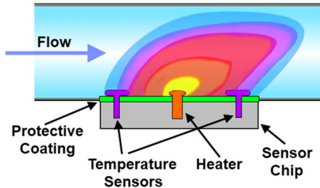
Fig. 2. Principle of operation for thermal mass flow sensor. Extracted from [18].
