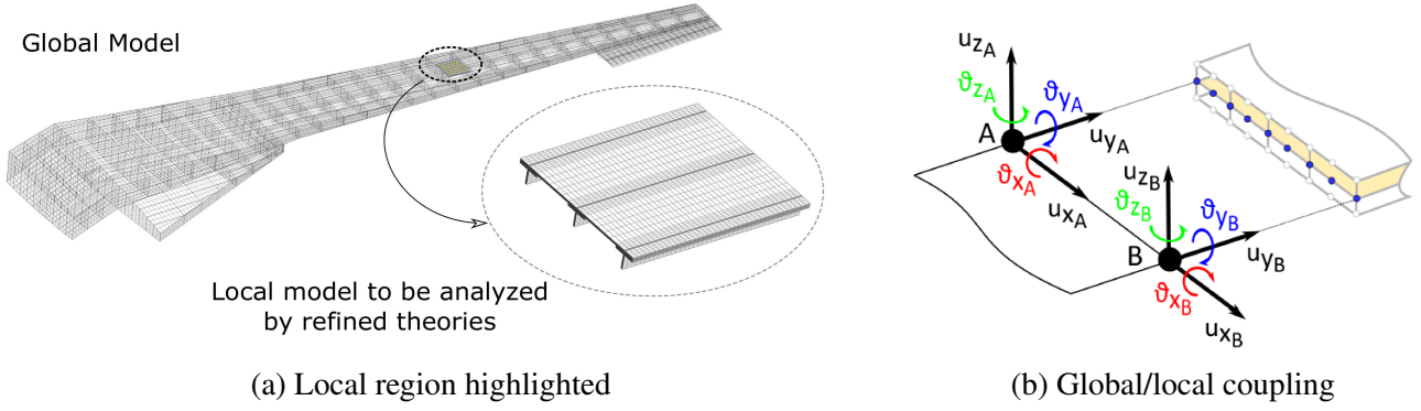
Fig. 1 : Schematic of proposed global/local analysis methodology.
