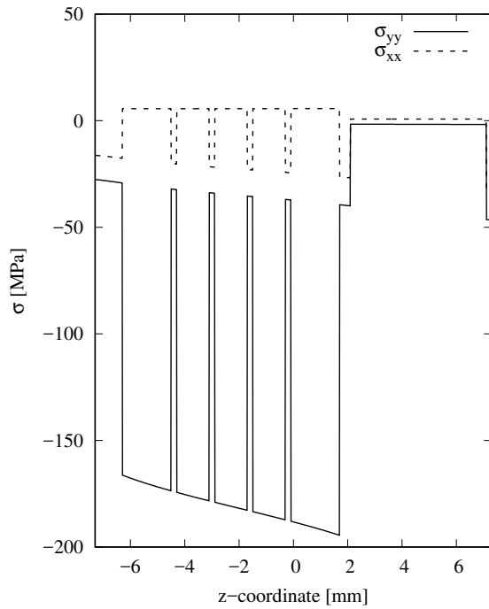
(a) In-plane normal stress
