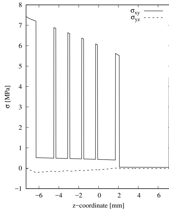
(b) In-plane and transverse shear
