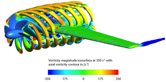
Fig. 6 Example of calculated isosurface of the vorticity magnitude behind the APIAN propeller with SRV and a Fokker 50 like half-wing colored by the level of the axial vorticity component.
