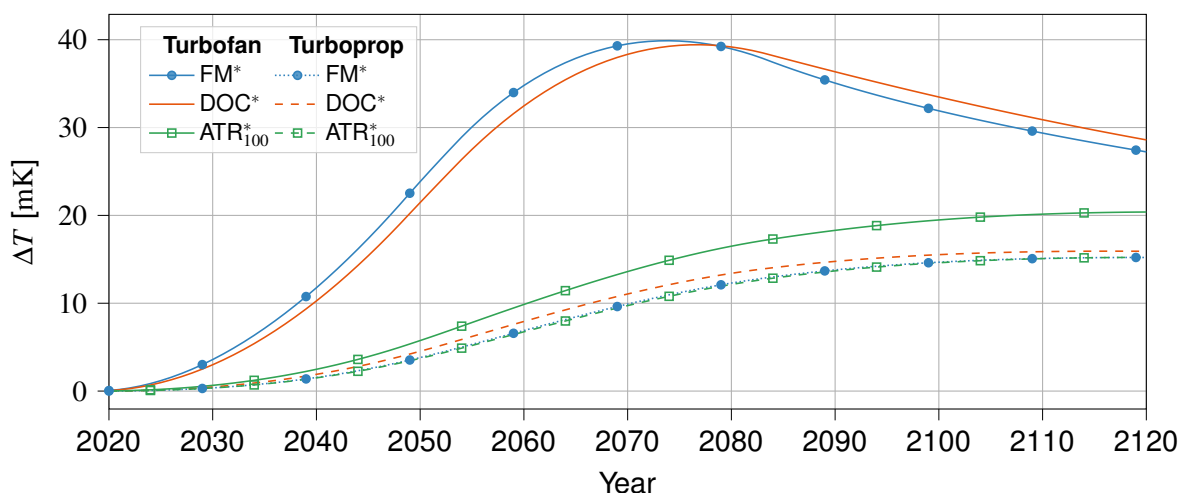
Figure 8 – Sea-level temperature change comparison between the turboprop aircraft with the block time constraint applied, and the turbofan aircraft
