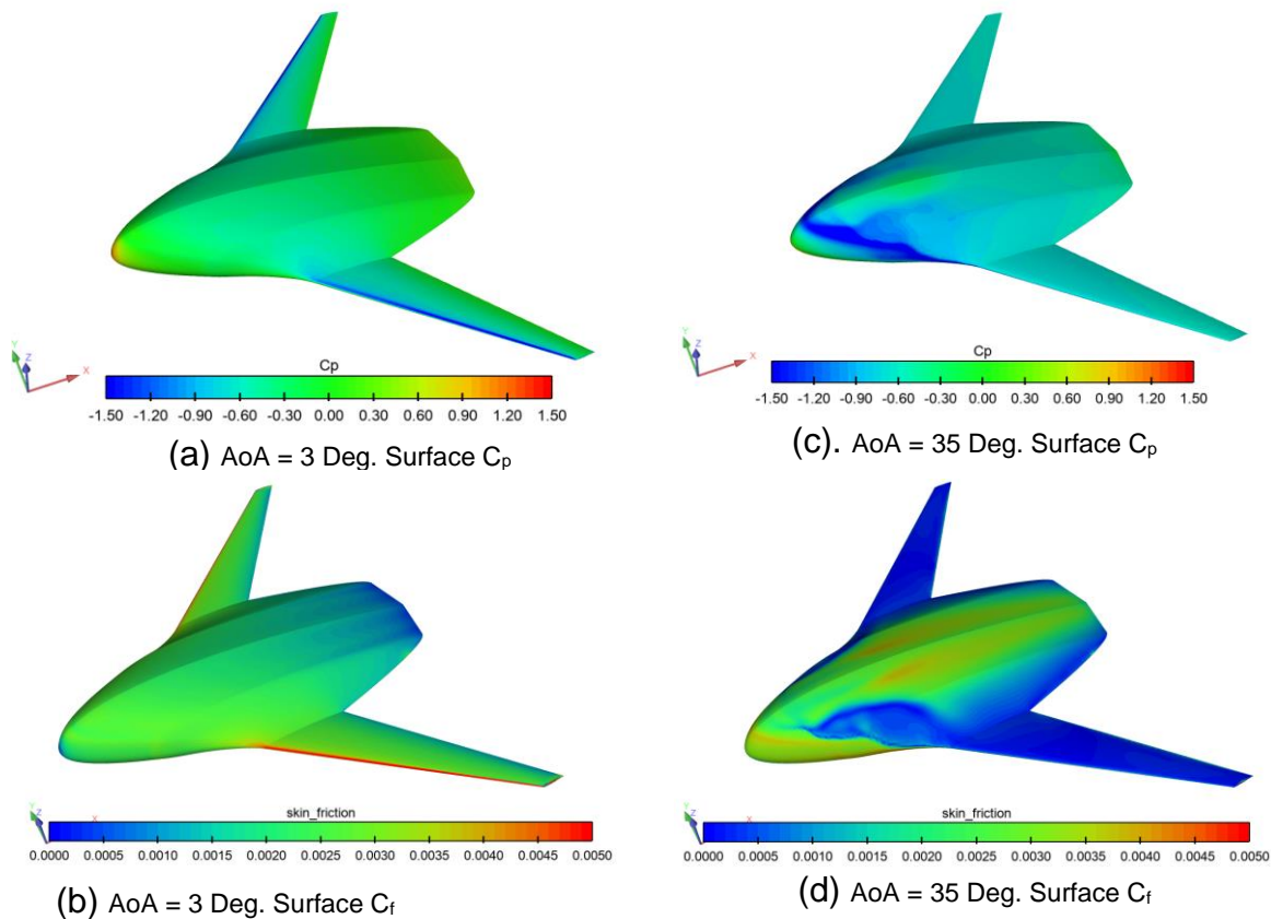
Figure 5: Examples of CFD simulations. Surface pressure and skin friction coefficients at AoA = 3 and AOA = 35 deg.
