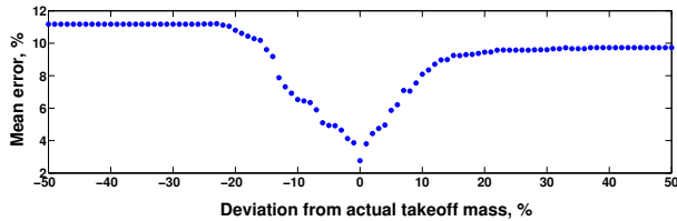
Fig. 3. B767-300: effect of deviation in takeoff mass on percentage mean error in predicted fuel flow rate on the modified test dataset in ascent. The results are from the LSB model.
