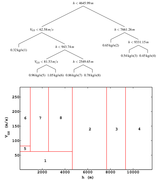
Fig. 1. A320-214: CART tree visualization in ascent: (top) the tree, and (bottom) the partitions of the predictor space induced by the tree. The numbers inside the partitions correspond to the leaf node numbers in the tree (written in parentheses for each leaf node).
