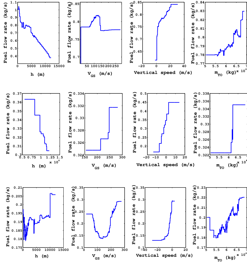
Fig. 2. A320-214: one variable partial dependence plots from the CART models: (top) ascent, (middle) cruise, and (bottom) descent.
