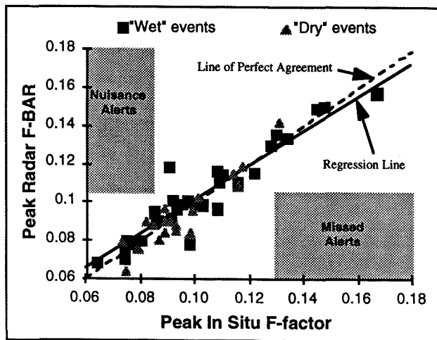
Figure 1 -- Radar Flight Test Performance
