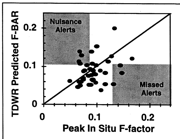
Figure 3 - TDWR Overall Flight Test Performance
