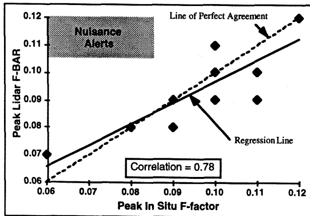
Figure 2 -- Lidar Flight Test Performance at Denver
