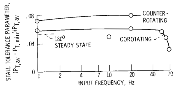
Figure 30. - Comparison of effects of rotating and 180° steady-state distortions on stall tolerance.
