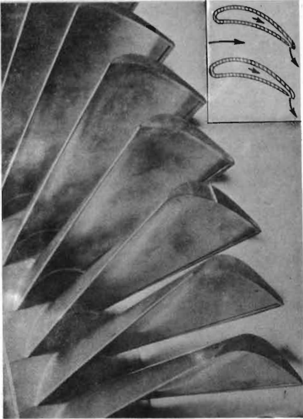
(B) JET-FLAP BLADE.
