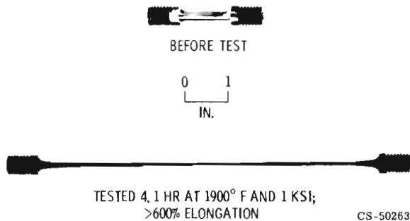
Figure 4. - Superplasticity in as-extruded TAZ-8A powder product.
