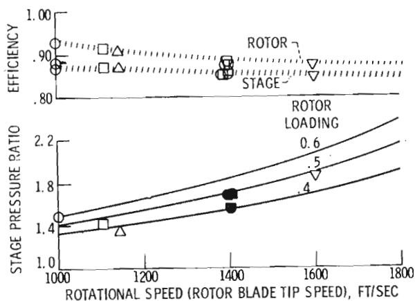
Figure 7. - Fan and compressor stage performance trends.
