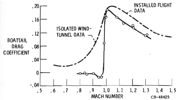
Figure 37. - Installation effect on boattail drag.
