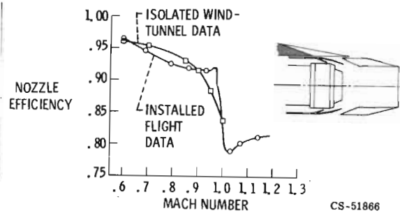
Figure 38. - Installation effect on auxiliary-inlet ejector.
