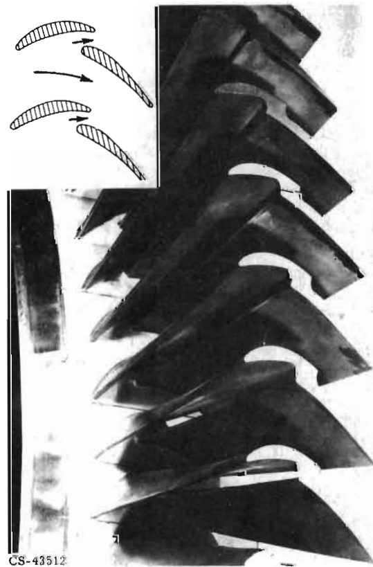
(A) TANDEM BLADE.
