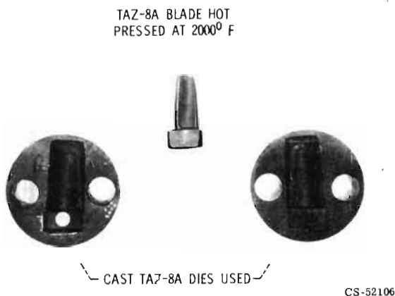
Figure 5. - Formability of TAZ-8A prealloyed powder product.
