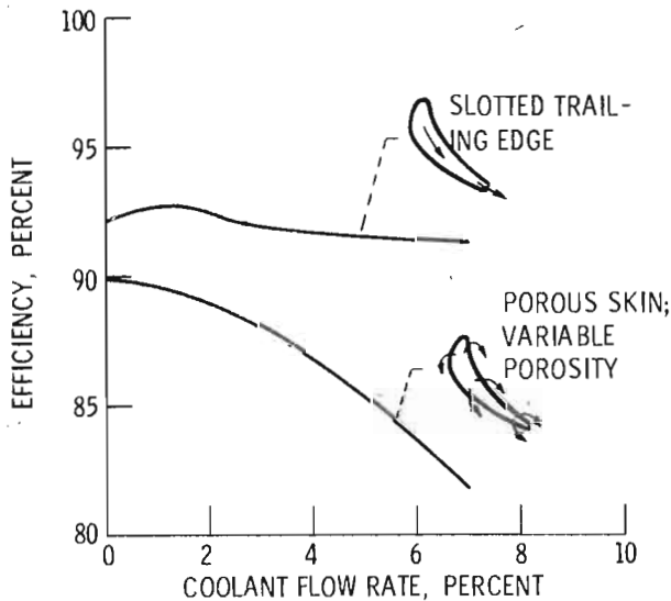
Figure 21. - Effect of coolant type on efficiency.
