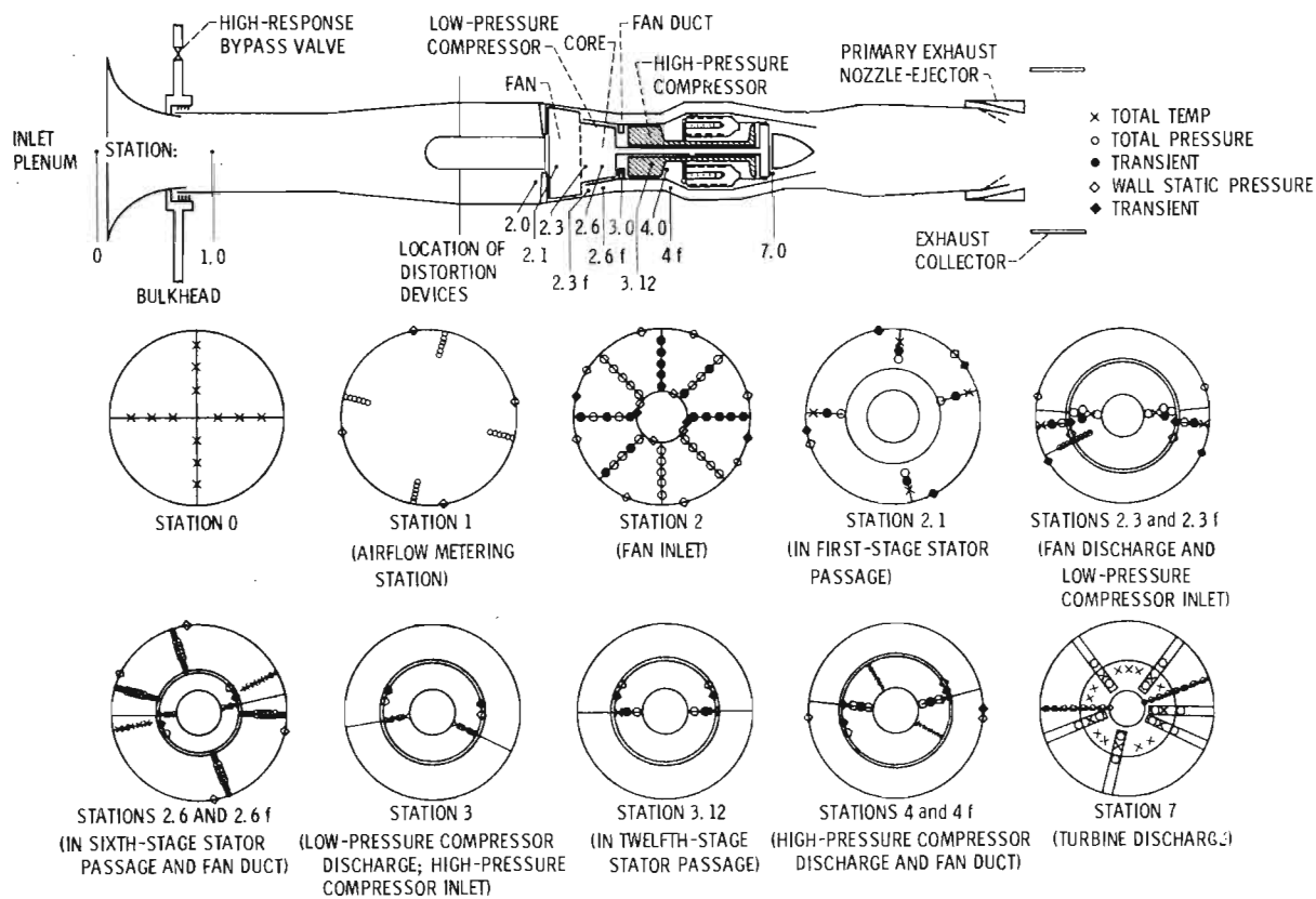
Figure 24. - Instrumentation layout.
