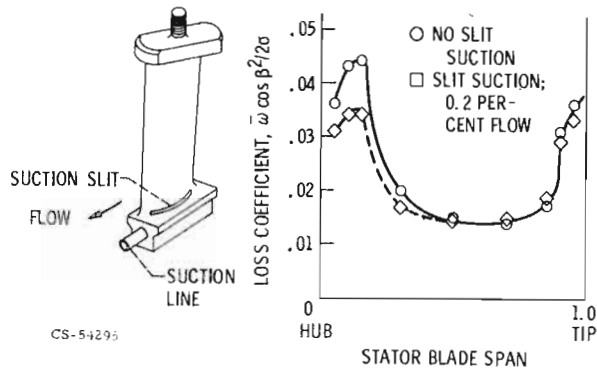
Figure 8. - Effect of slit suction on stator losses.
