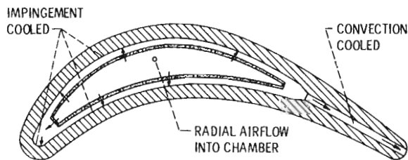
Figure 19. - Impingement cooled turbine blade configuration.
