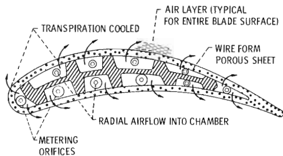
(B) TRANSPARATION COOLED.
