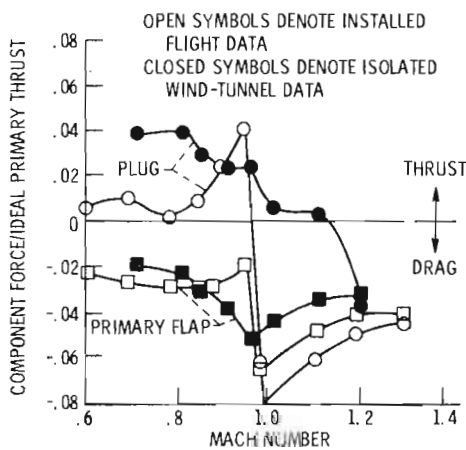
Figure 41. - Installation effect on conical-plug and primary-flap forces.
