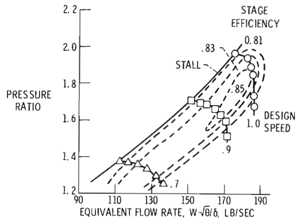
Figure 10. - Transonic fan stage performance.
