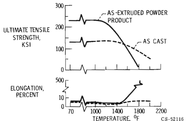
Figure 3. - Improvements in tensile properties of TAZ-8A.
