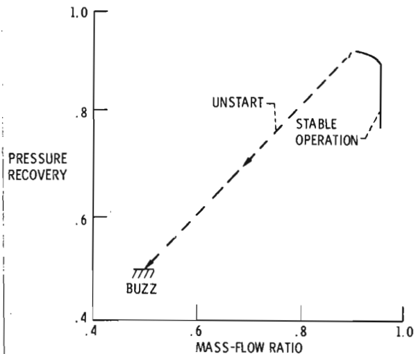
Figure 31. - Mixed compression inlet.
