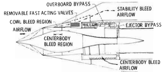
(A) CROSS SECTION OF 60-40 STABILITY INLET.
