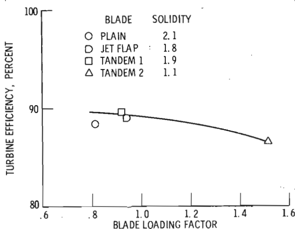
Figure 23. - Performance of turbines with highly loaded blades.
