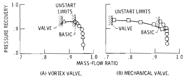
Figure 34. - Valve effects on inlet performance.
