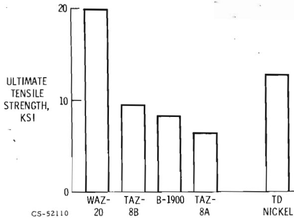
Figure 1. - Strength of nickel-base alloys at 2200° F.
