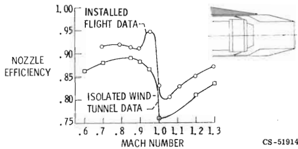
Figure 36. - Installation effect on variable-flap ejector.
