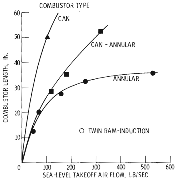
Figure 15. - Comparison of combustor lengths.
