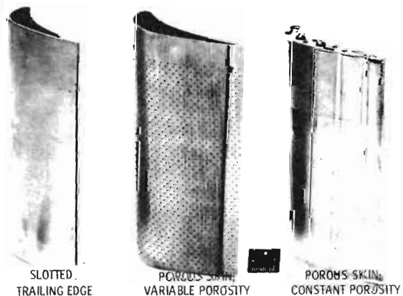
Figure 20. - Example stator vanes tested.
