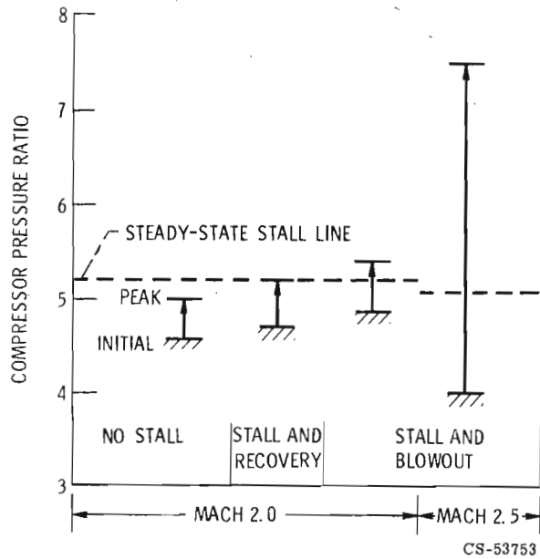
Figure 32. - Inlet unstart effect on engine.
