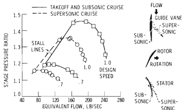
Figure 11. - Fan stage performance with variable camber vanes.
