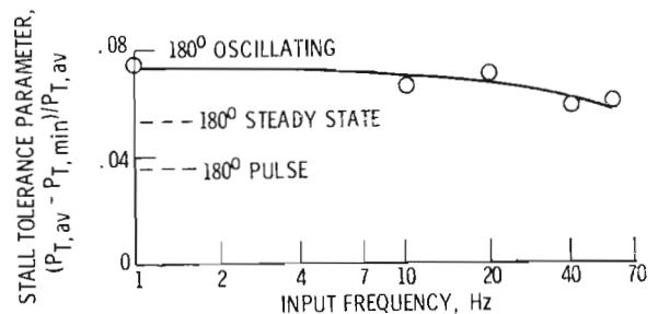
Figure 29. - Comparison of effects of steady-state, oscillating, and pulse 180° distortions on stall tolerance.
