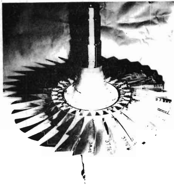
Figure 9. - Highly loaded transonic compressor rotor. Blade tip speed, 1600 feet per second.
