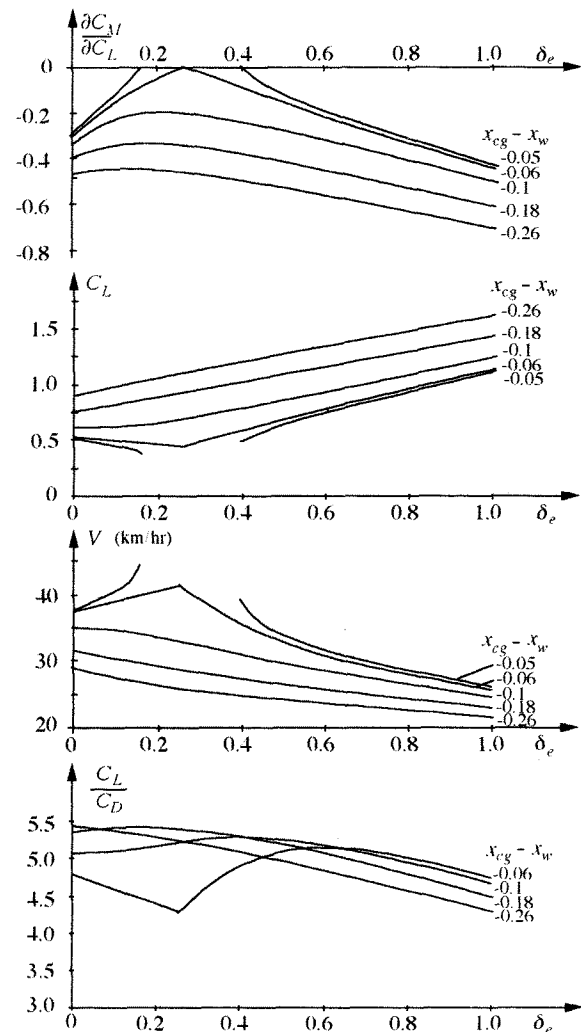
Figure 3 - Trim conditions as functions of elevons deflection. Model B.
