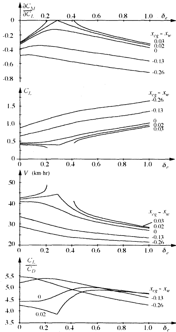
Figure 2 - Trim conditions as functions of elevons deflection. Model A.
