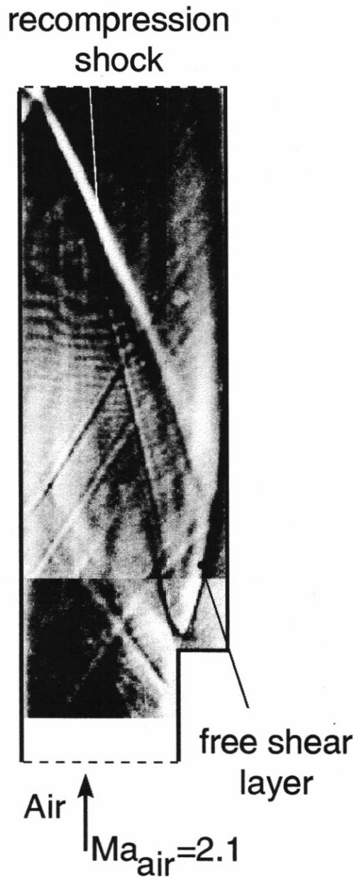
Fig. 1: Flow structure of a supersonic flow over a rearward facing step at Ma_{air} = 2.1
