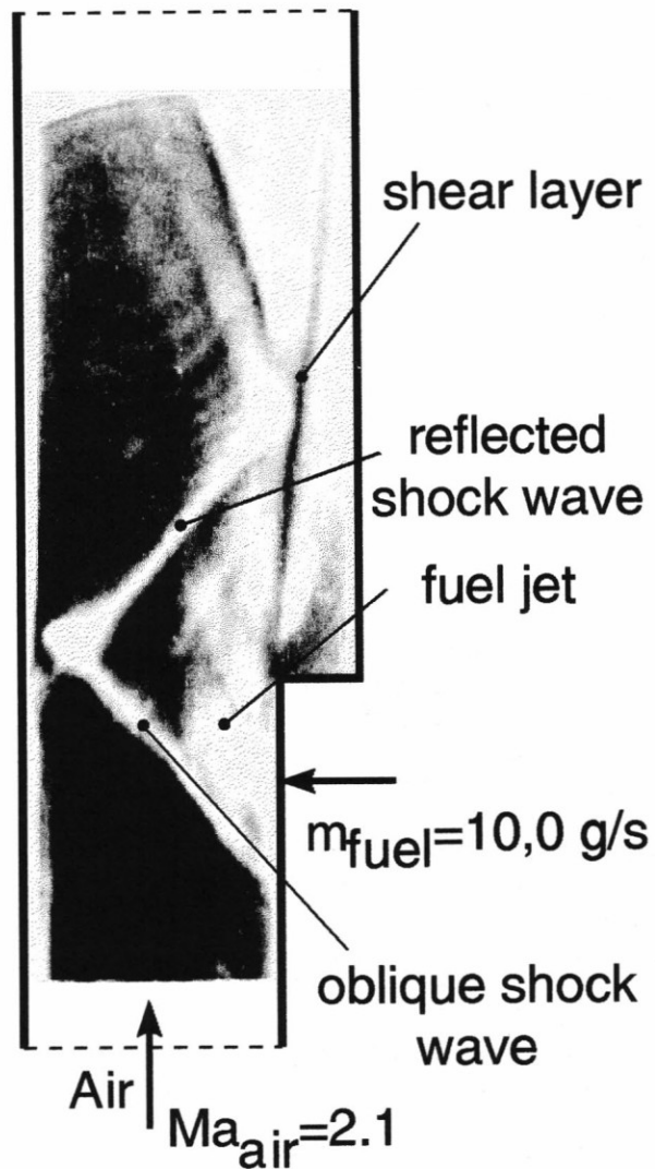
Fig. 2: Supersonic flow field with fuel injection ( Ma_{air} = 2.1 ; m_{fuel} = 10,0 \text{ g/s} )
