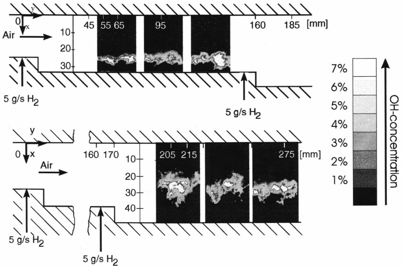
Fig. 10: Turbulent flame structure in the wake of the first and second recirculation zone monitored by means of laser induced fluorescence ( Ma_{air}=2.1 ; m_{H_2}= 10.0 g/s; multistep injection, four holes)
