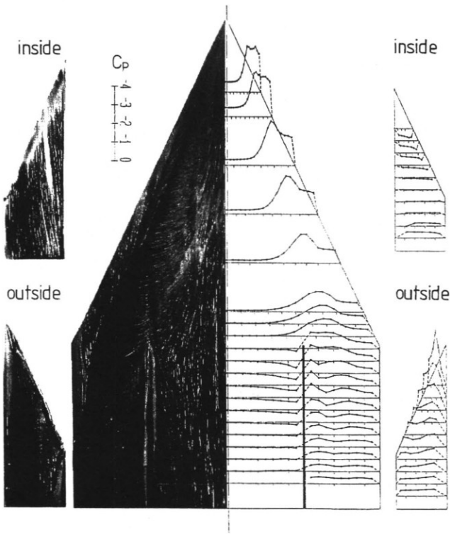
Fig. 12: Pressure distribution and surface oilflow pattern on the wing-fin configuration SH at \alpha = 20^\circ , \beta = 0^\circ (Oilflow patterns from the fin enlarged).
