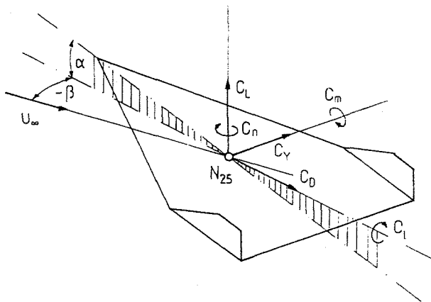
Fig. 4: Experimental coordinate system for windtunnel data reduction.
