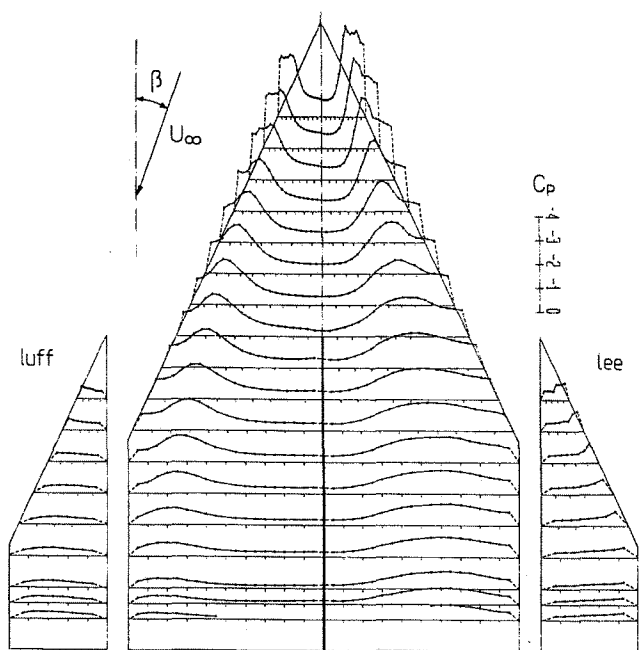
Fig. 10: Pressure distribution on the wing-fin configuration MC at \alpha = 25^\circ , \beta = 10^\circ .
