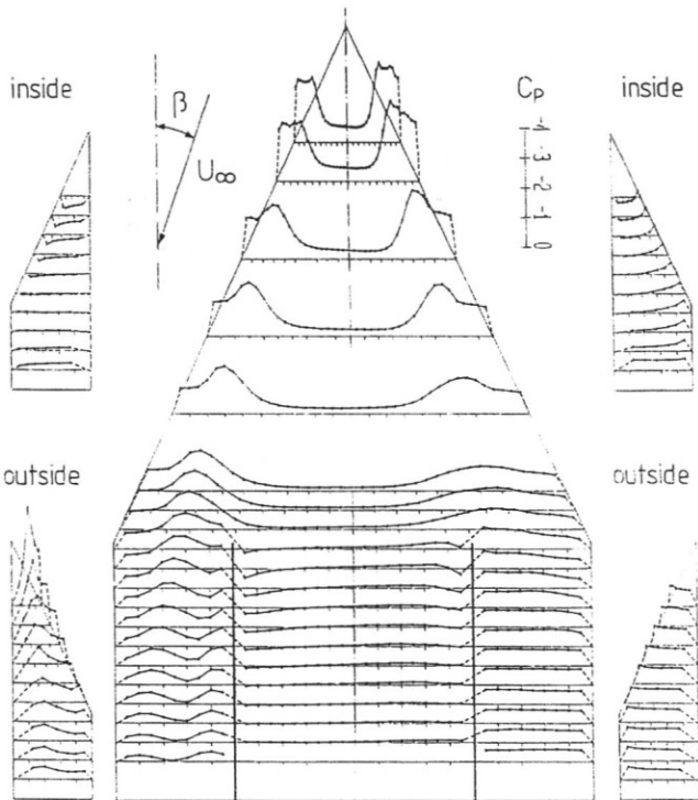
Fig. 13: Pressure distribution on the wing-fin configuration SH at \alpha = 20^\circ , \beta = 5^\circ .
