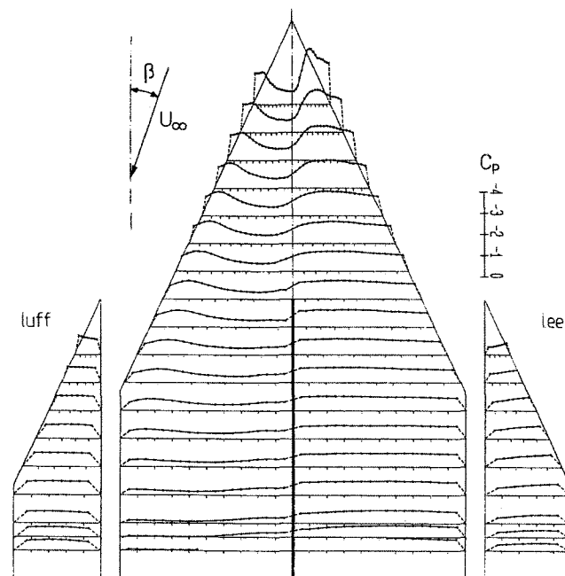
Fig. 11: Pressure distribution on the wing-fin configuration MC at \alpha = 25^\circ , \beta = 20^\circ .
