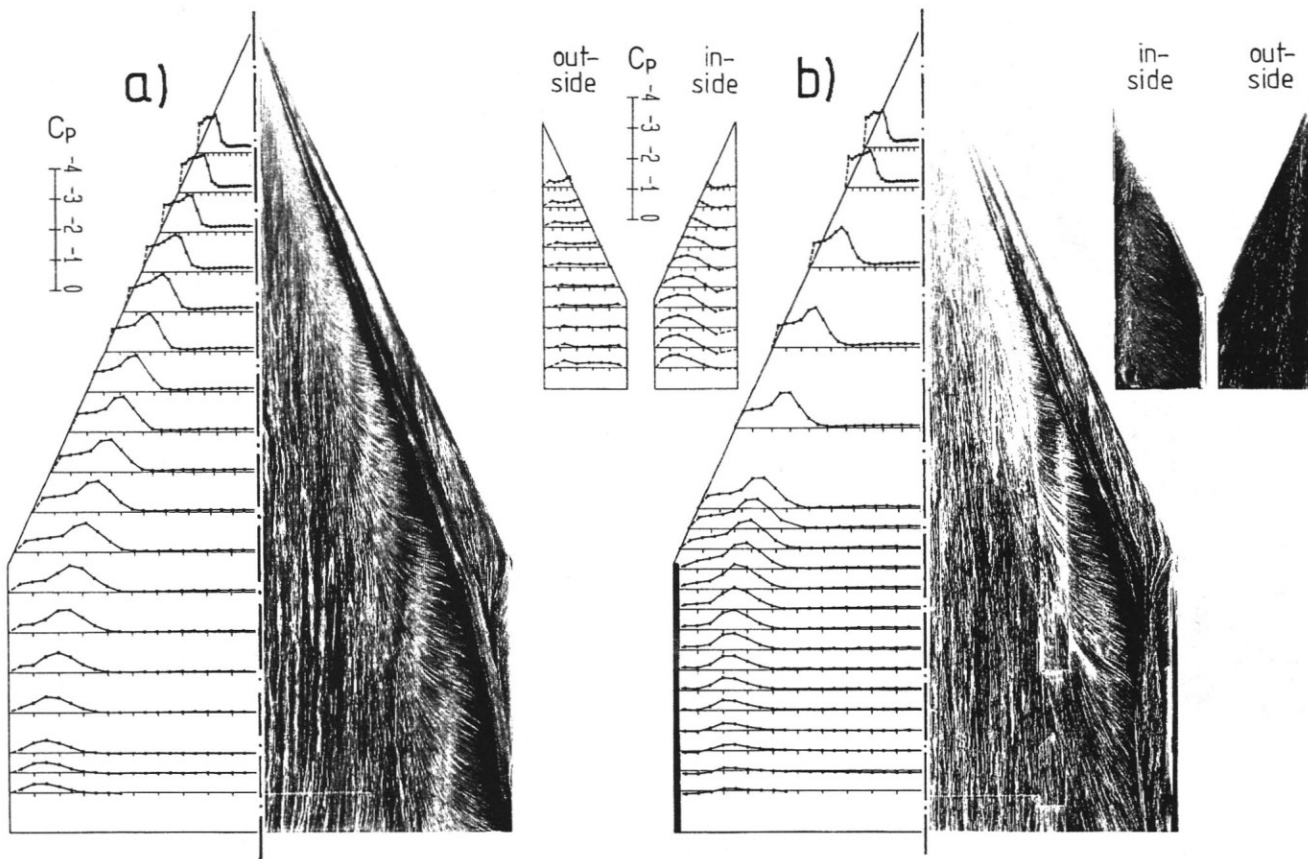
Fig. 15: Pressure distribution and surface oilflow pattern at \alpha = 10^\circ , \beta = 0^\circ for a) Wing alone (W) and b) Wing-fin configuration ST (Oilflow patterns from the fin enlarged).
