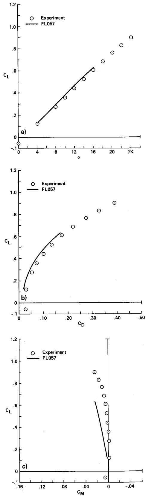
Figure 20. Experiment-CFD forces and moments for wing/body/chine, M_\infty = 1.6 ; a) lift curve, b) drag polar, c) moment curve
