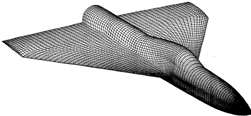
Figure 2. Generic fighter wing/body surface grid, 134 \times 49 \times 65 points
