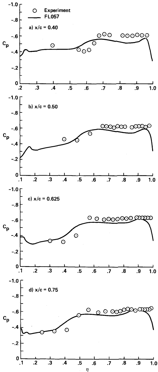
Figure 17. Upper surface pressure distributions for wing/body/chine, M_\infty = 1.4 , \alpha = 20.0^\circ
