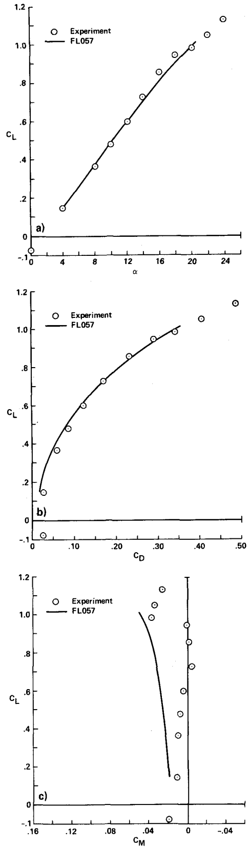
Figure 16. Experiment-CFD forces and moments for wing/body/chine, M_\infty = 1.2 ; a) lift curve, b) drag polar, c) moment curve
