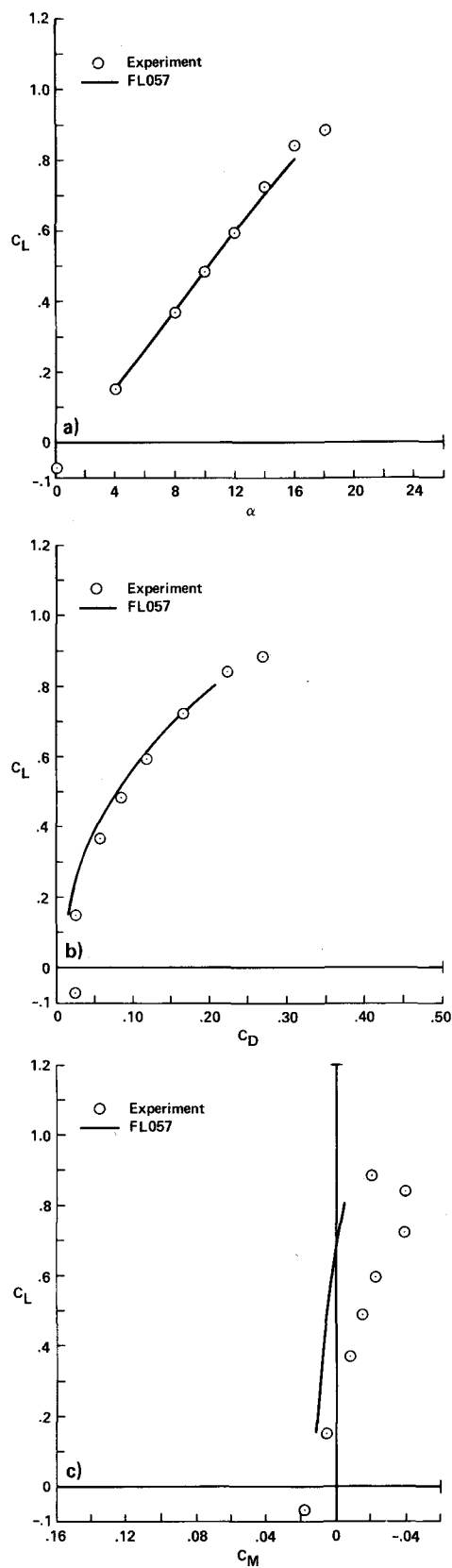
Figure 14. Experiment-CFD forces and moments for wing/body, M_\infty = 1.2 ; a) lift curve, b) drag polar, c) moment curve
