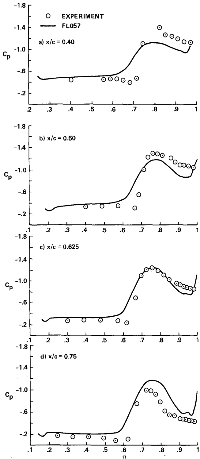
Figure 11. Upper surface pressure distributions for wing/body/chine, M_\infty = 0.8 , \alpha = 12.0^\circ
