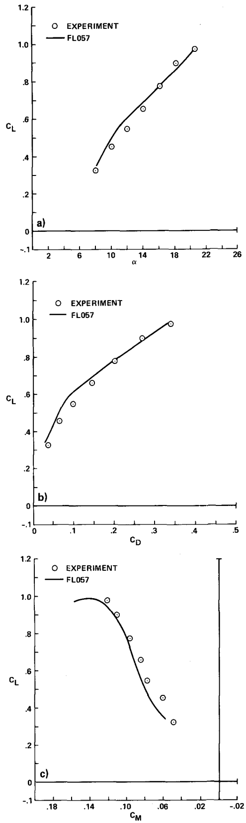
Figure 12. Experiment-CFD forces and moments for wing/body/chine, M_\infty = 0.8 ; a) lift curve, b) drag polar, c) moment curve
