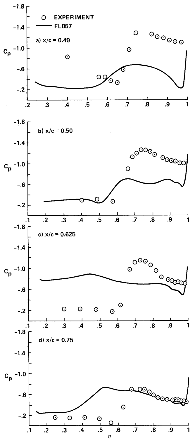
Figure 9. Upper surface pressure distributions for wing/body, M_\infty = 0.8 , \alpha = 12.0^\circ
