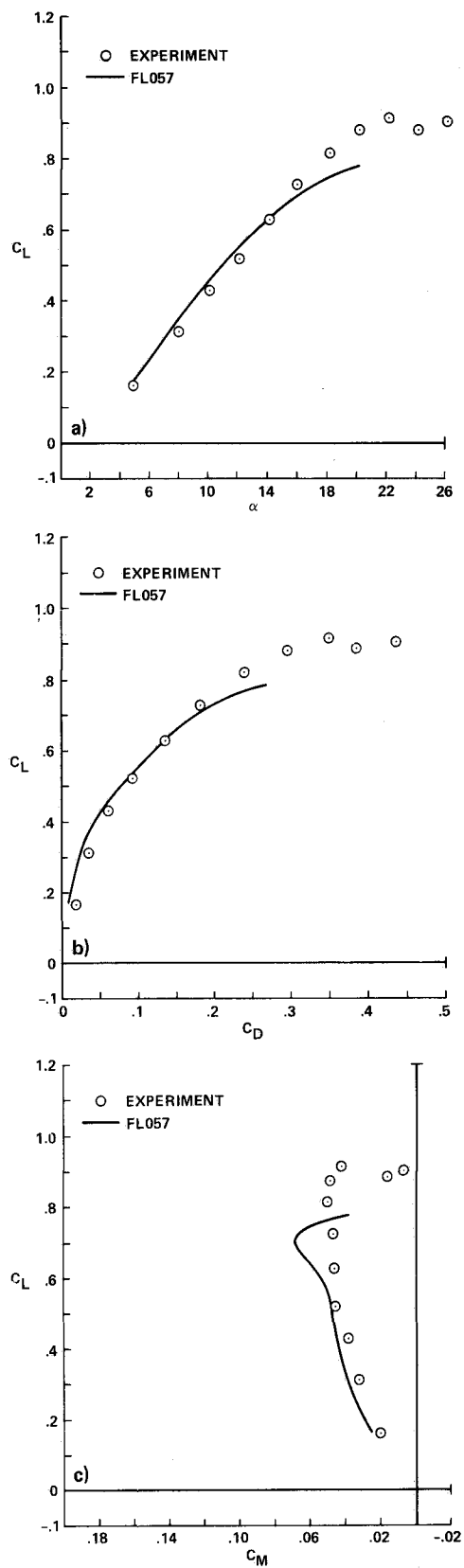
Figure 10. Experiment-CFD forces and moments for wing/body, M_\infty = 0.8 ; a) lift curve, b) drag polar, c) moment curve
