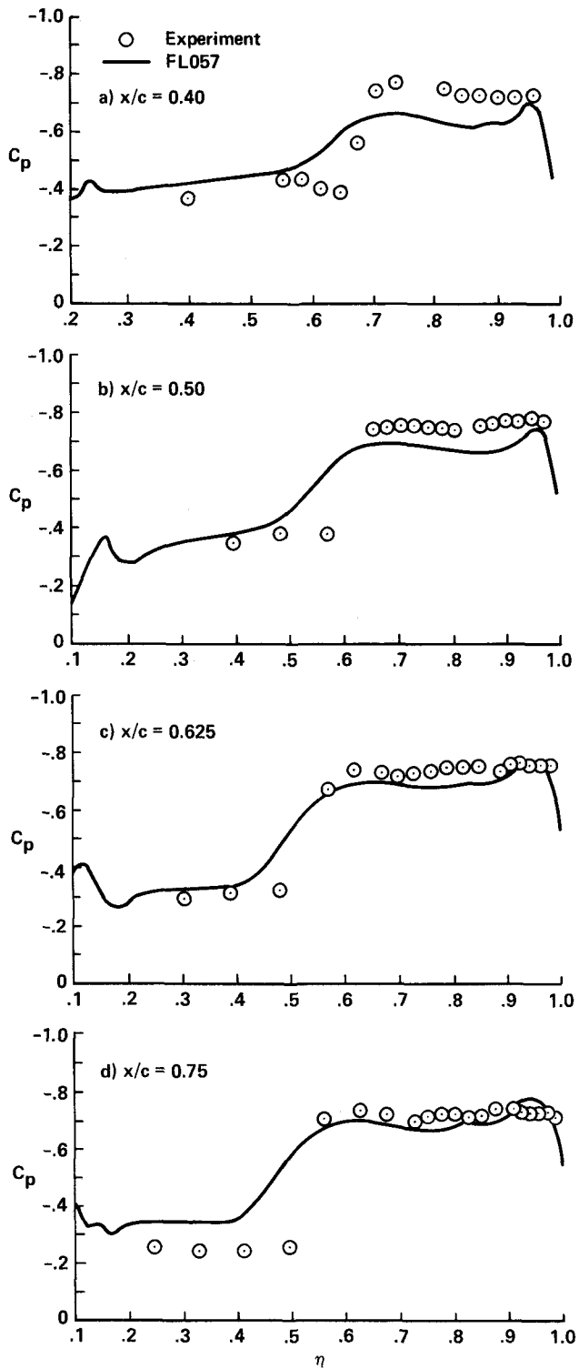
Figure 15. Upper surface pressure distributions for wing/body/chine, M_\infty = 1.2 , \alpha = 16.0^\circ
