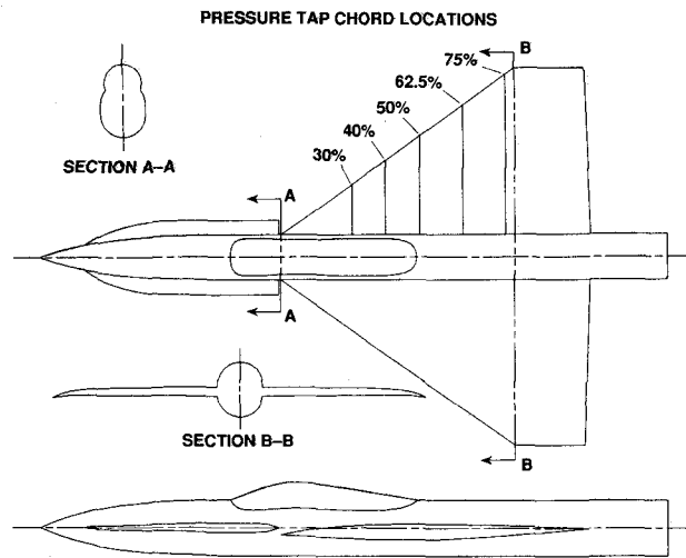
Figure 1. Generic fighter with chine
