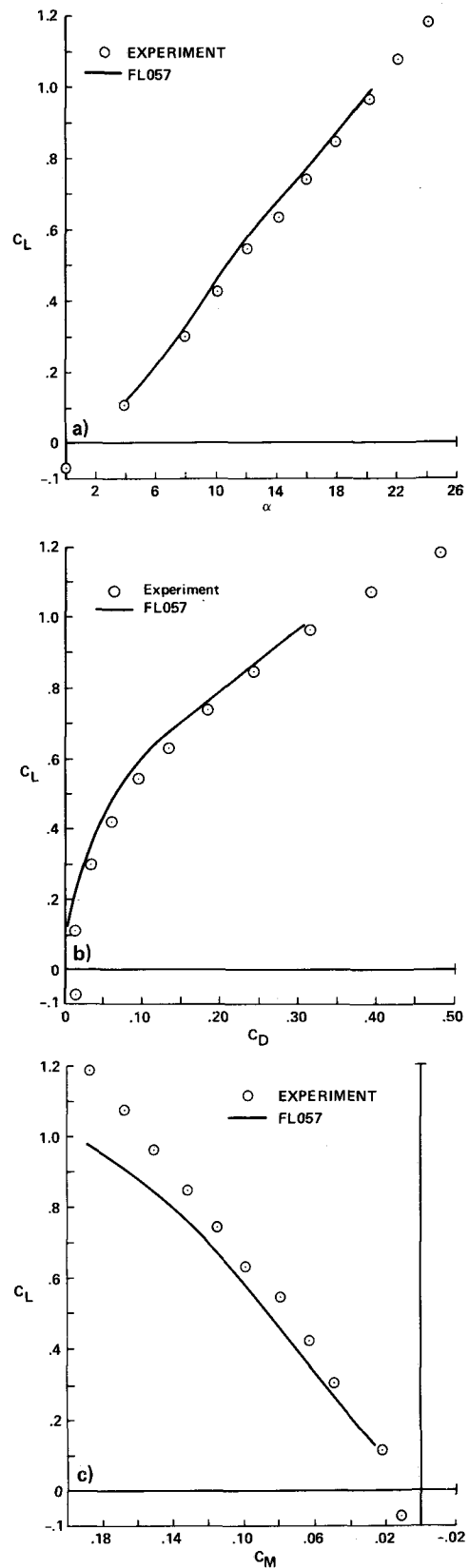
Figure 8. Experiment-CFD forces and moments for wing/body/chine, M_\infty = 0.6 ; a) lift curve, b) drag polar, c) moment curve
