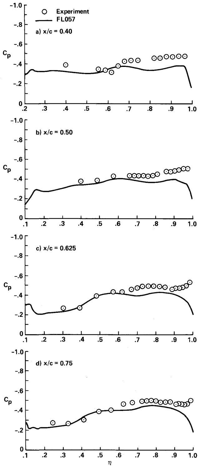
Figure 19. Upper surface pressure distributions for wing/body/chine, M_\infty = 1.6 , \alpha = 16.0^\circ
