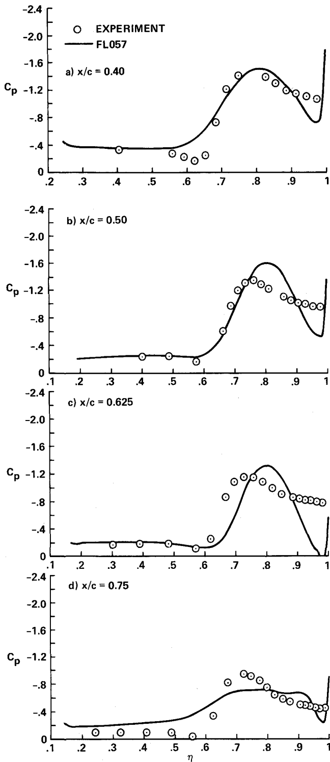
Figure 5. Upper surface pressure distributions for wing/body, M_\infty = 0.6 , \alpha = 12.0^\circ
