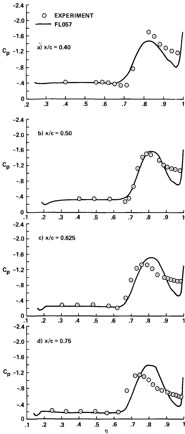
Figure 7. Upper surface pressure distributions for wing/body/chine, M_\infty = 0.6 , \alpha = 12.0^\circ
