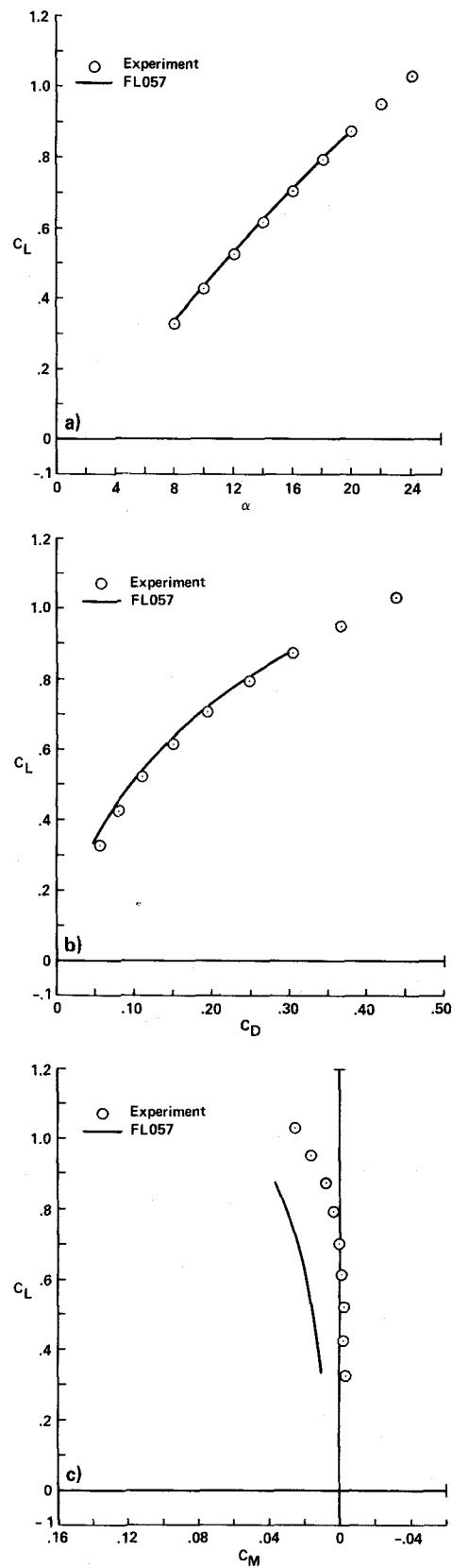
Figure 18. Experiment-CFD forces and moments for wing/body/chine, M_\infty = 1.4 ; a) lift curve, b) drag polar, c) moment curve
