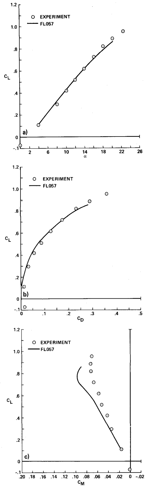
Figure 6. Experiment-CFD forces and moments for wing/body, M_\infty = 0.6 ; a) lift curve, b) drag polar, c) moment curve
