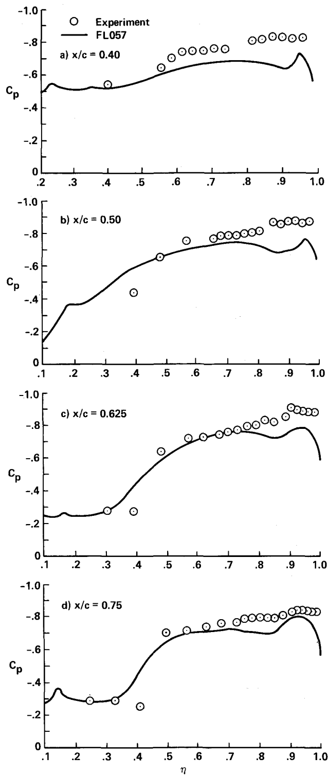
Figure 13. Upper surface pressure distributions for wing/body, M_\infty = 1.2 , \alpha = 16.0^\circ
