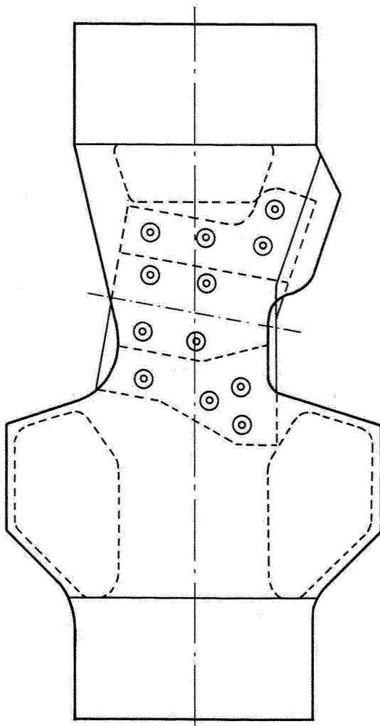
Fig. 3 Fatigue test specimen representing critical wing root lower skin area of NF-5A/B aircraft (from ref. 2)
