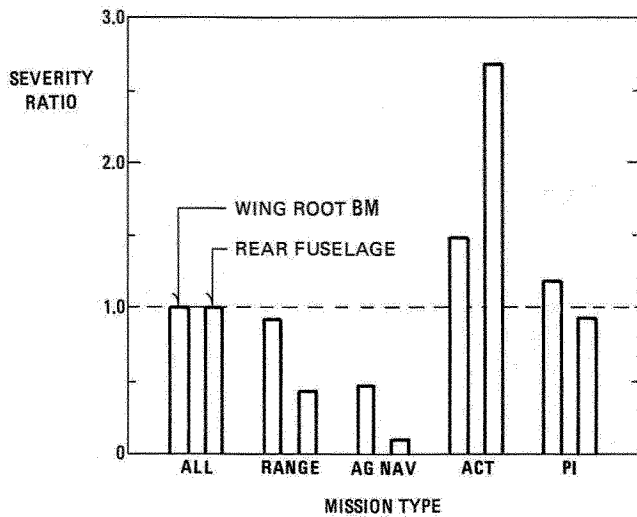
Fig. 5 Relative severities of different mission types (from ref. 4)
