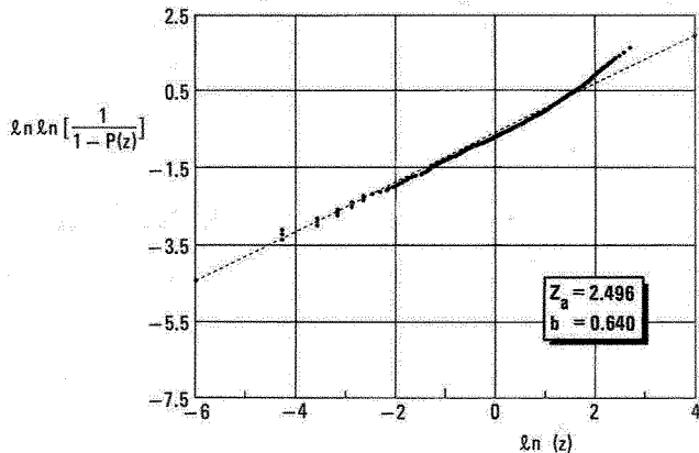
Fig. 1 Best fit Weibull distribution. For all Strike flights (R=0.984) (from ref. 1)
