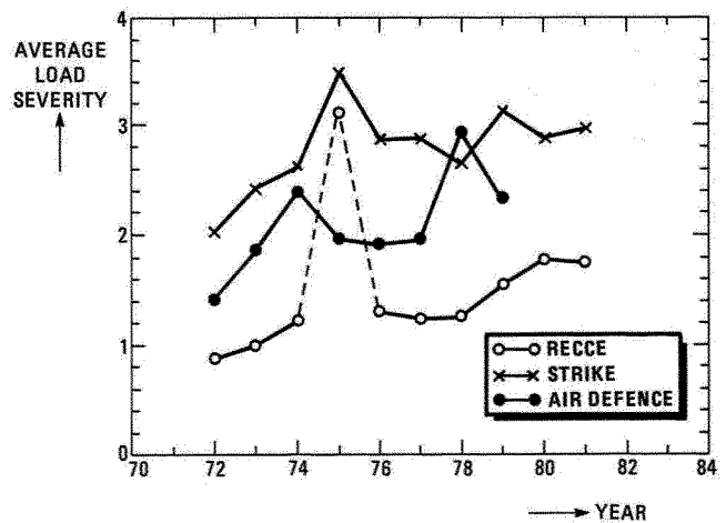
Fig. 4 The annually recorded load severity LSF for the three different duties of RNLA F-104G (from ref. 3)
