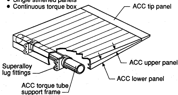
Figure 5. Control surface concept.
