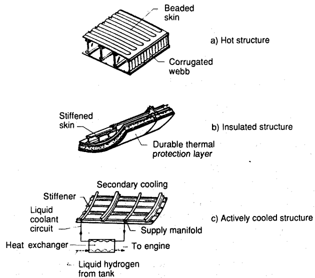
Figure 3. Typical airframe structural concepts.
