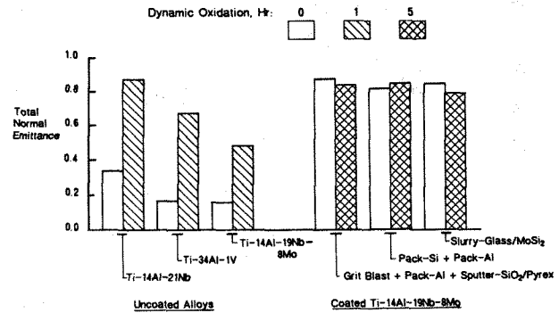
Figure 28. Total normal emittance at 1800°F.
