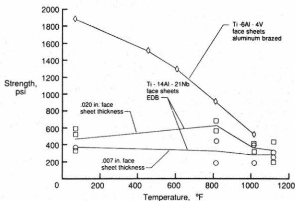
Figure 27. Flatwise tension strength of honeycomb-core sandwich specimens.
