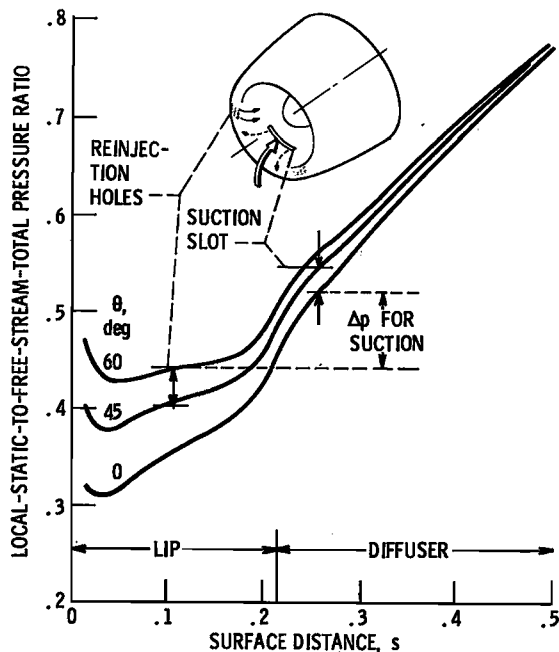
Figure 10. - Self-pumping boundary-layer-control system.
