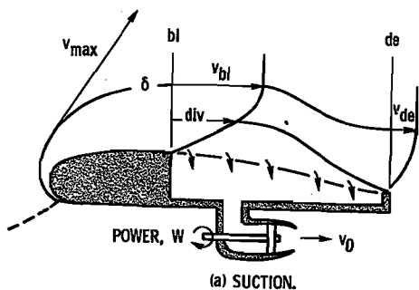
(a) SUCTION.
