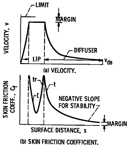
Figure 4. - Optimum flow distributions for inlets without boundary-layer control.
