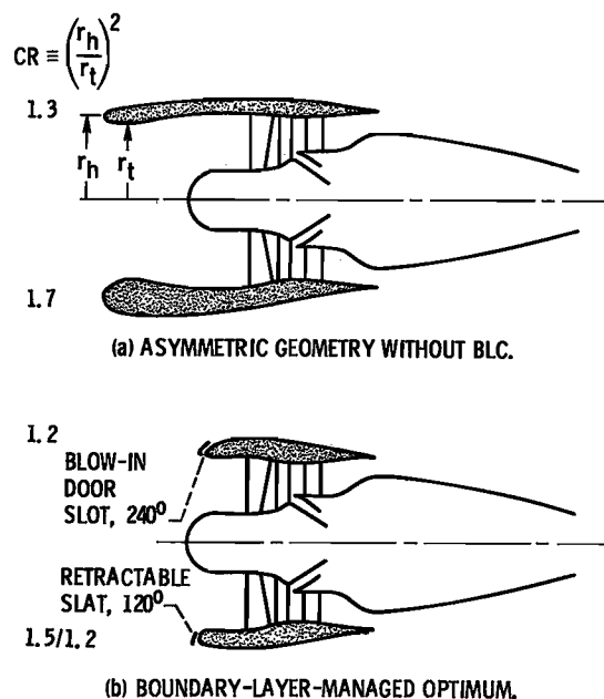
Figure 17. - Comparison of subsonic high-angle-of-attack nacelles.
