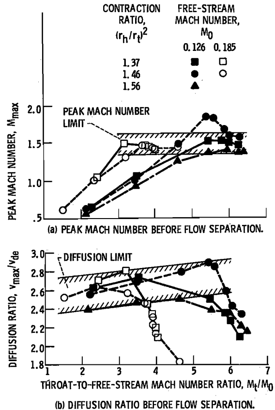
Figure 5. - Experimental separation data for inlets. (From ref. 6.)
