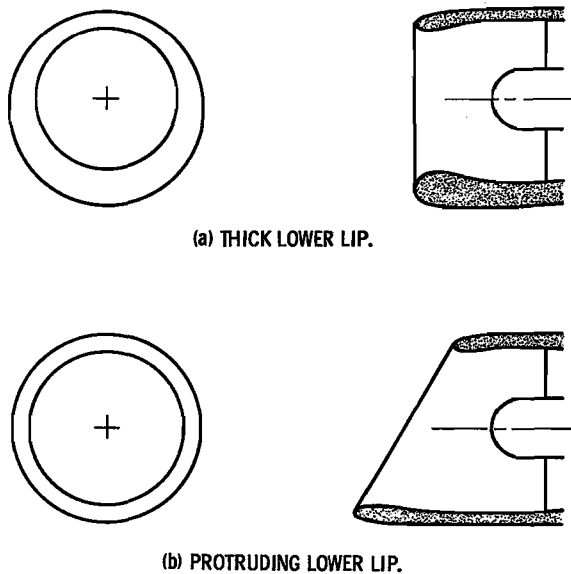
Figure 6. - Low-speed, high-angle-of-attack inlets without boundary-layer control.
