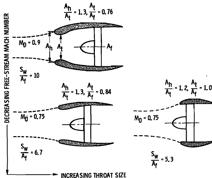
Figure 15. - Effect of free-stream Mach number and inlet throat size on nacelle wetted area.
