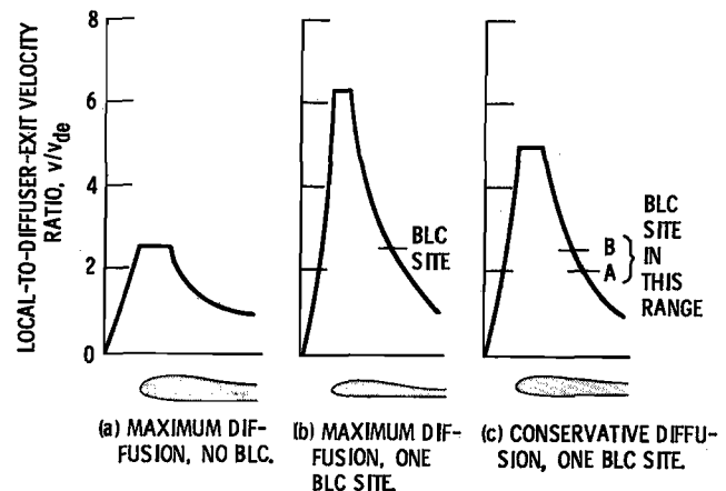
Figure 7. - Optimum inlet velocity distributions with boundary-layer control.
