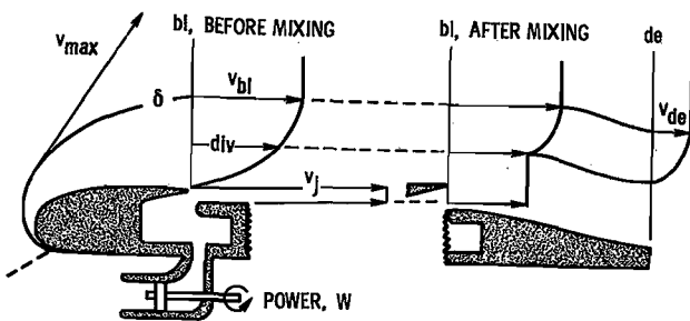
(b) BLOWING.
