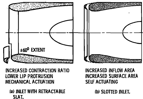
Figure 12. - Inlets with boundary-layer management.
