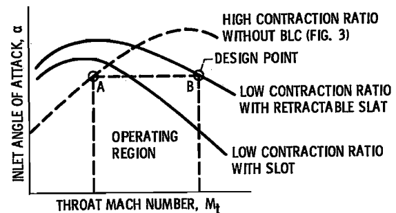
Figure 14. - Review of inlet design-point selection.
