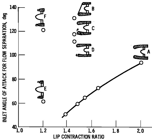
Figure 13. - Summary of experimental results for high-angle-of-attack inlets. M_0 = 0.13 ; M_t = 0.45 .
