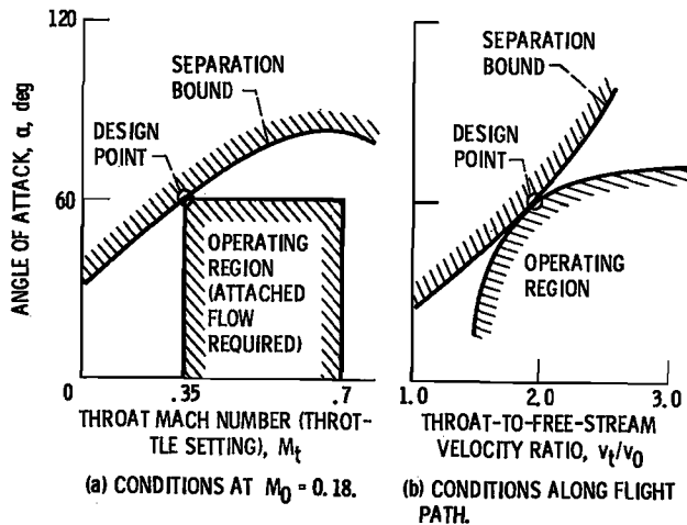
Figure 3. - Initial design-point selection.
