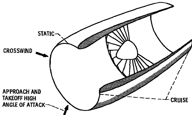
Figure 2. - Critical nacelle regions.
