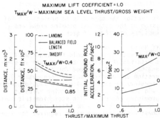
Figure 20. Estimate of Field Length and Takeoff Acceleration
