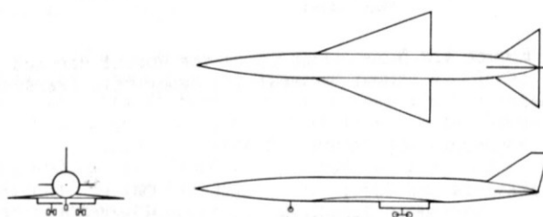
Figure 2. Wing-Body Configuration
