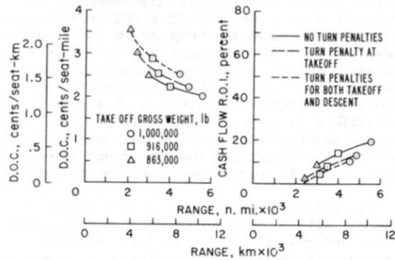
Figure 22. Effect of Turns to Avoid Overland Sonic Boom on HST Economics
