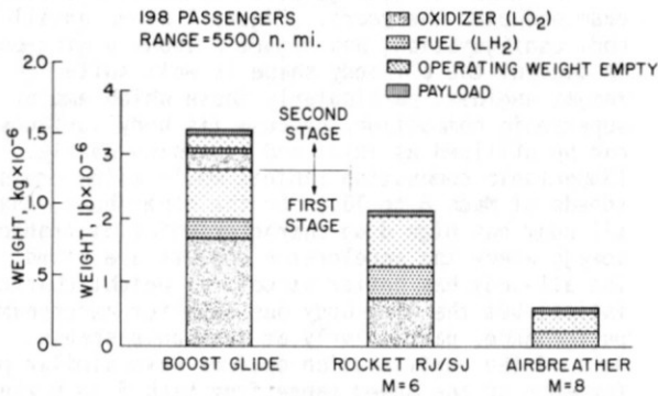
Figure 3. Weight Breakdown for Rocket Boosted and Airbreathing Hypersonic Transports
