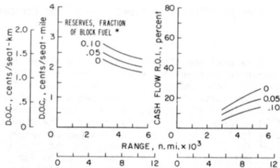
Figure 10. Effect of Fuel Reserve Requirements on HST Economics
