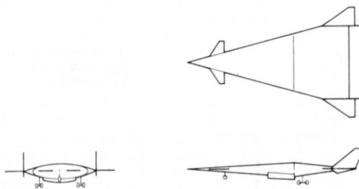
Figure 1. All-Body Configuration
